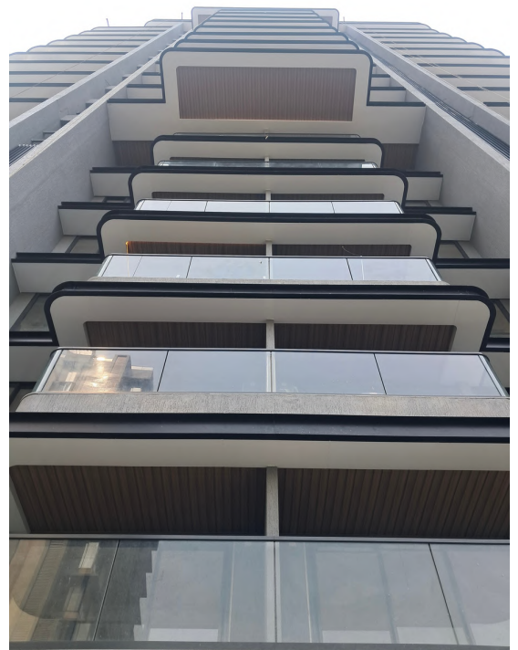
EVERGREEN, BANDRA Precision-fabricated chajja system comprising CNC-cut C-channels with ACP cladding.
