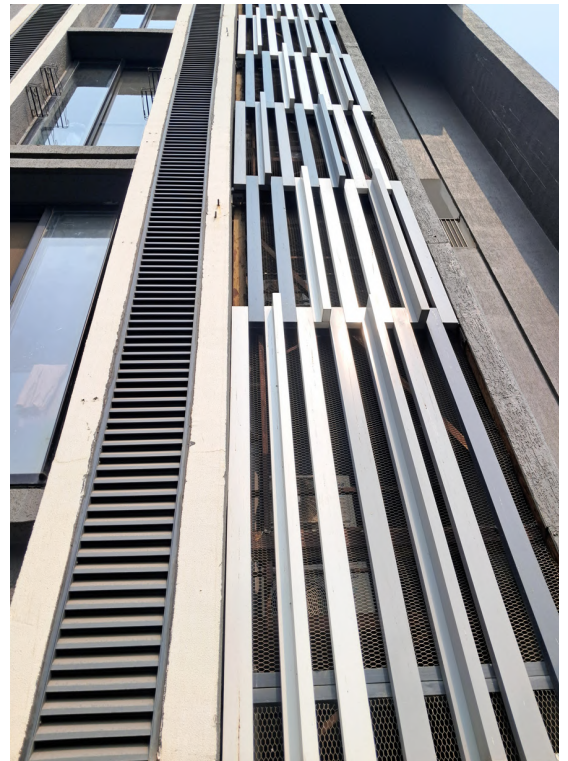
NEW LIGHT, KHAR Custom duct fin systems with integrated normal fins and detailed projections. (Outside View)
