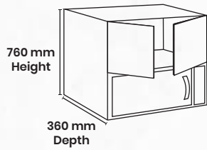
Upper Cabinet with appliances
