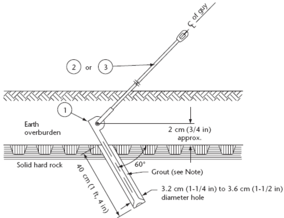
Figure 2 Rock anchor with earth overburden
