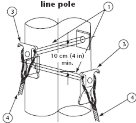
Figure 5 V-guy
