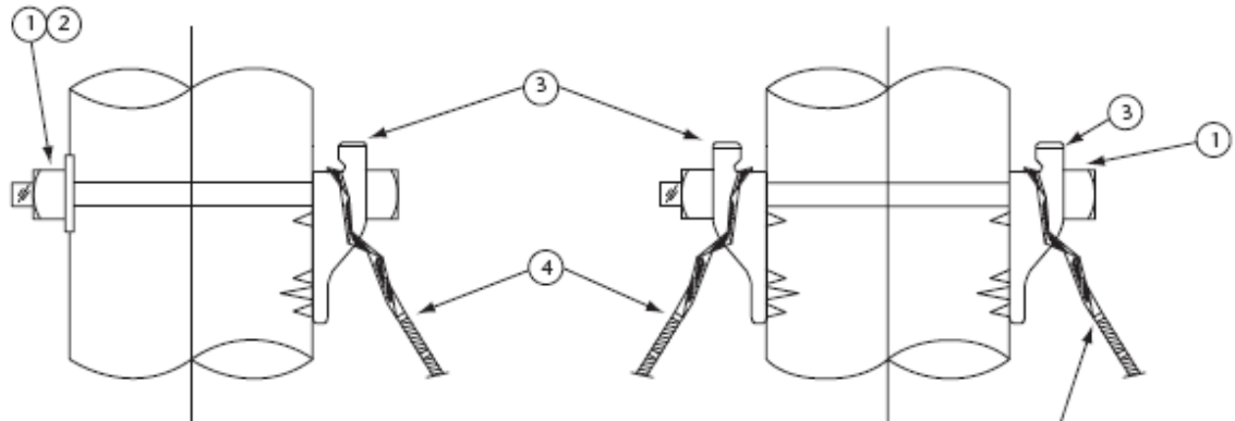
Figure 1 Single guy
