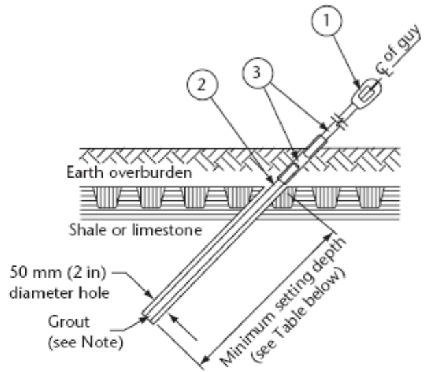
Figure 2 Shale and limestone anchor with earth overburden
