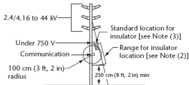
Down guy
