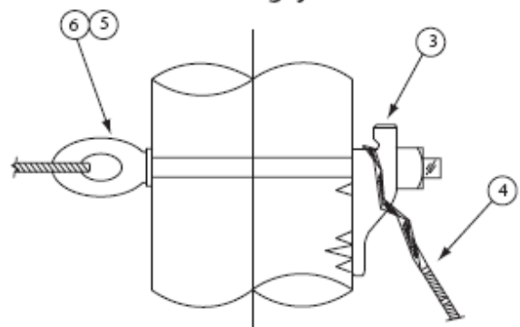
Figure 4 Span and anchor guy stub pole
