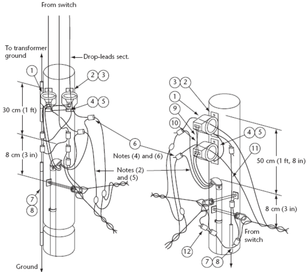
Figure 1 Transformer pole
