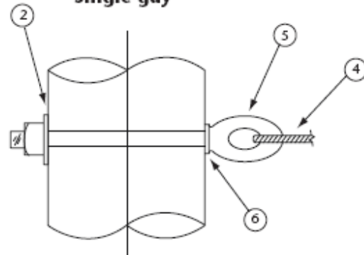
Figure 3 Span and anchor guy line pole
