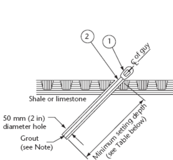
Figure 1 Shale and limestone anchor without earth overburden
