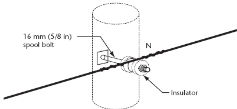
Figure 2 Neutral spool Tangent (0° to 3°)
