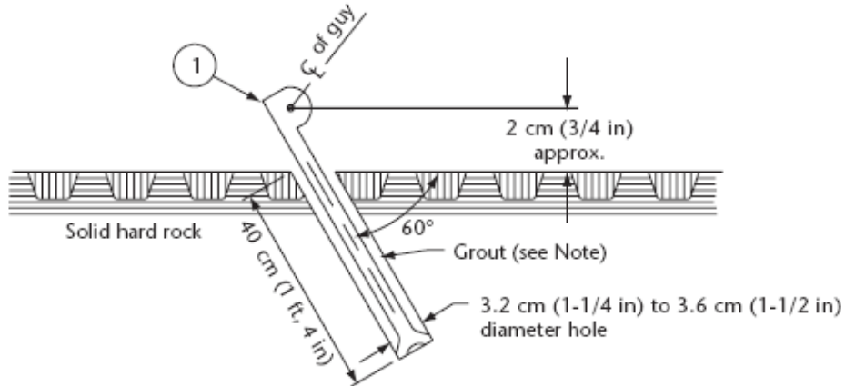
Figure 1 Rock anchor without earth overburden
