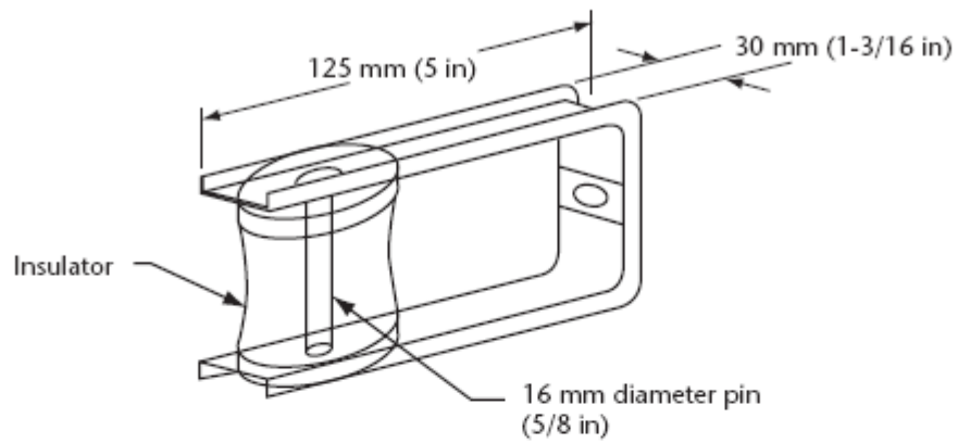
Figure 1 One-wire rack (Neutral spool)
