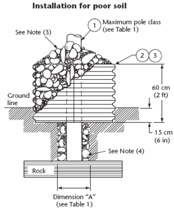
Figure 2 Overburden up to 18 in short of normal soil setting depth (shown)
