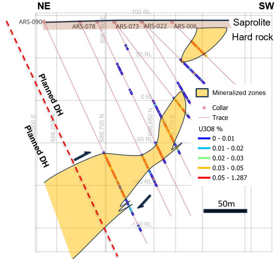
Cross Section through the mineralized vein
