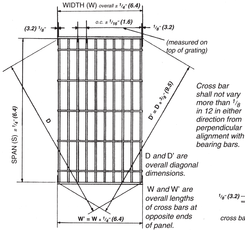
overall dimensions and squareness
