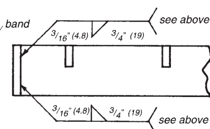
WELDING DETAIL
