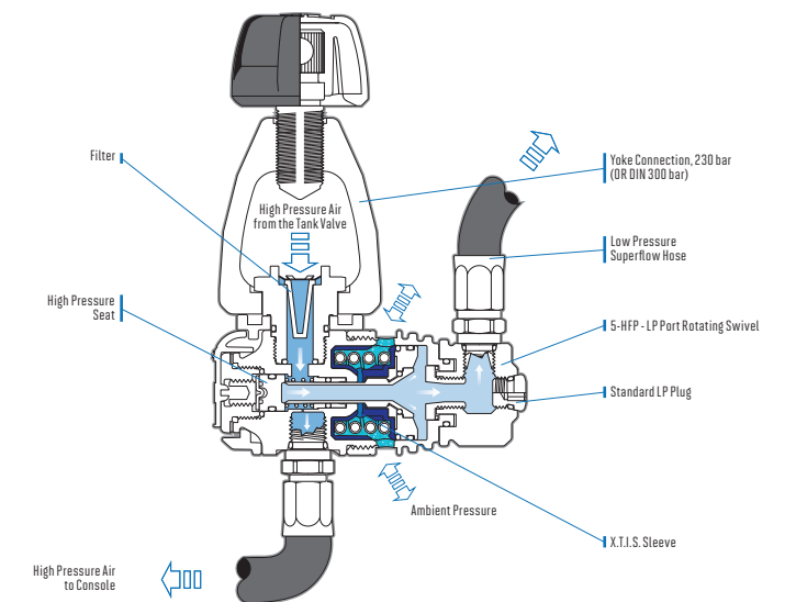
MK25 EVO DIAGRAM
