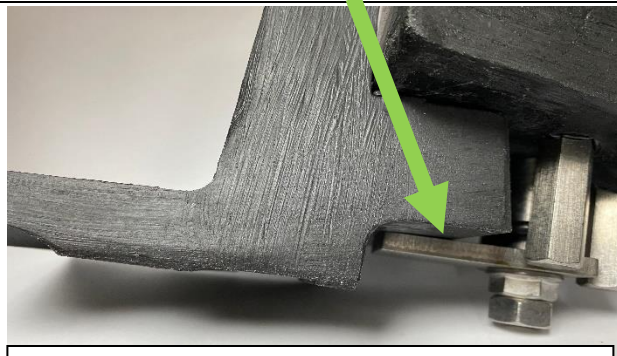
Frame/Cover Cross Section – Paddle Lock Latch Engaged
