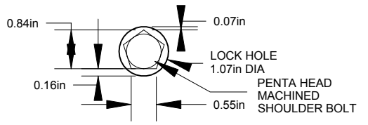
HOLE TO BOLT CLEARANCES
