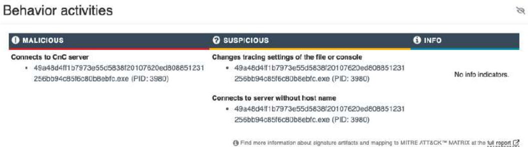
Figure 4.20 – The high-level overview within the Any.Run report
