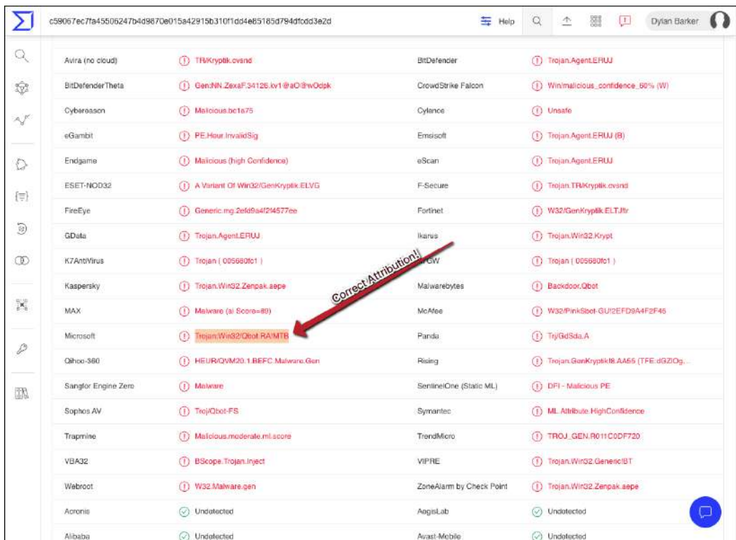
Figure 2.12 – Scan results of highly similar files that have been submitted to VirusTotal
