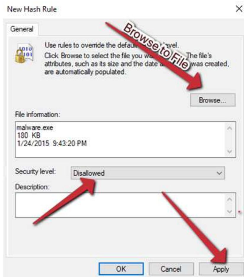
Figure 9.6 – Applying the hash rule by browsing to the offending file
