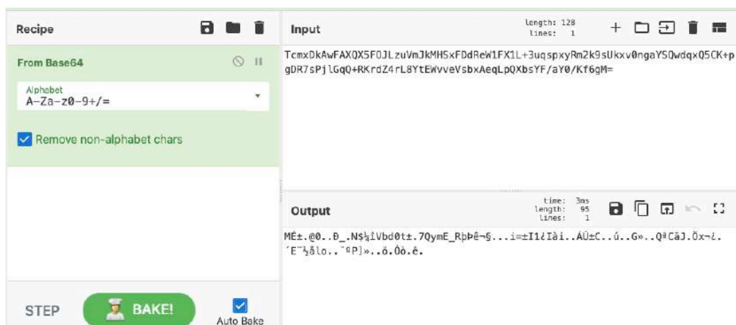
Figure 8.14 – Binary data from a Base64-encoded string in CyberChef
