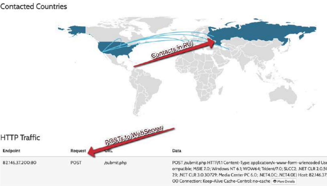
Figure 4.12 – A Geo-IP world map of network connections made by the sample
