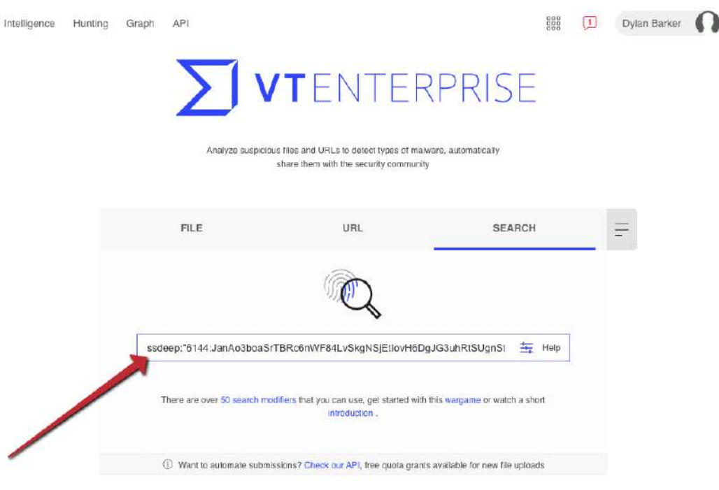
Figure 2.10 – ssdeep search syntax on VirusTotal
