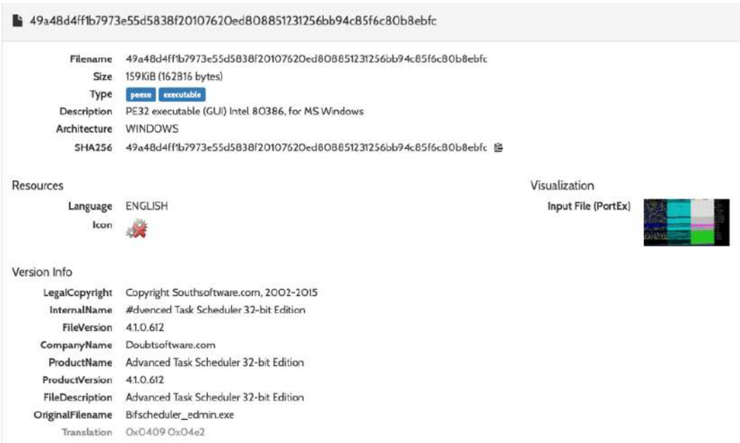
Figure 4.9 – Static file information in HybridAnalysis
