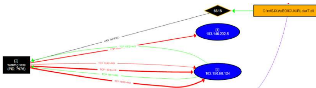
Figure 6.39 – ProcDOT showing the injection process and C&C communication from WerMgr
