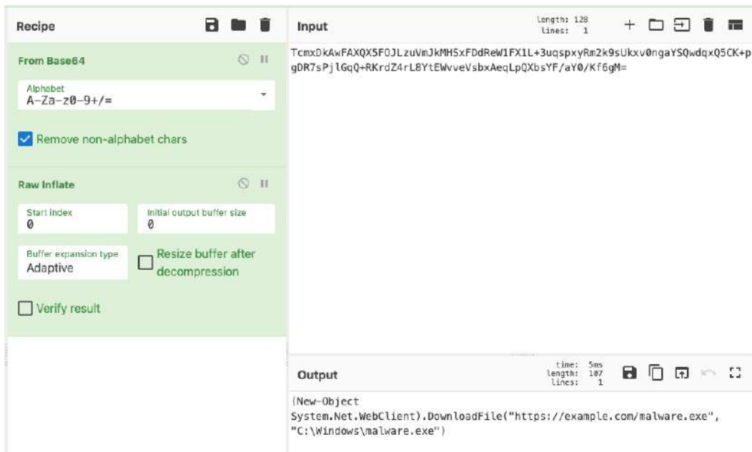
Figure 8.15 – Inflating the binary data from within CyberChef to return the ASCII command
