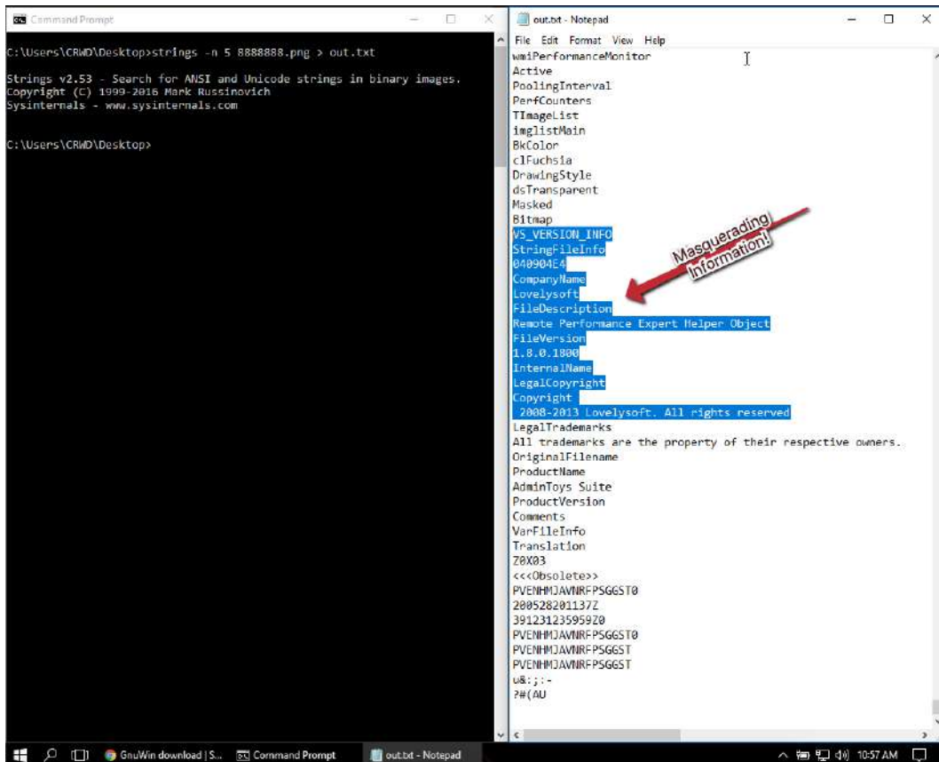
Figures 2.16 – Output of strings showing modules imported from the Windows API, as well as information on which executable may have served as the basis of this payload
