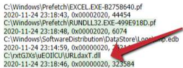
Figure 6.36 – Obviously malicious DLLs dropped to disk
