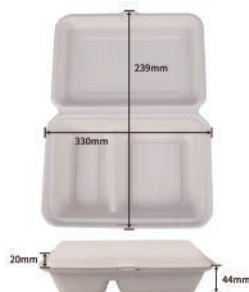
1000 ml 2 compartments hinged box
