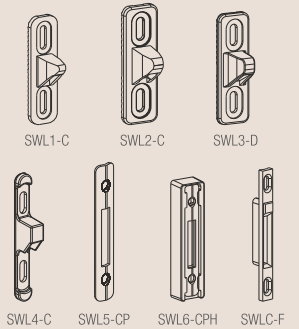
22 SLIDING WINDOW LATCH
