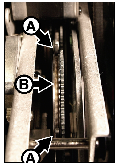
Figure 21: Gobo clip
