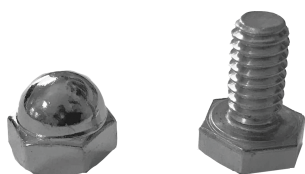
Smaller Bolt and Acorn Nut (6) - attaches seat back to stanchions. Bolt size is 1/4 -20 x 1".
