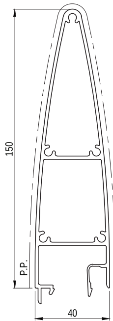
EP13373 40mm BOX LOUVRE BULLNOSE Paint Perimeter: 321mm Anodised Perimeter: 481mm
