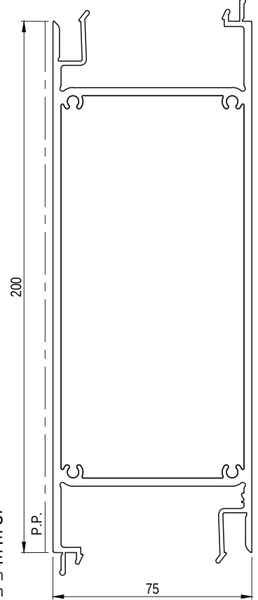
EP15125 75mm INTERMEDIATE BOX LOUVRE Paint Perimeter: 570mm Anodised Perimeter: 855mm
