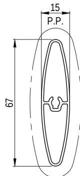
EPD0262 67mm ELLIPTICAL BLADE Paint Perimeter: 144mm Anodised Perimeter: 144mm
