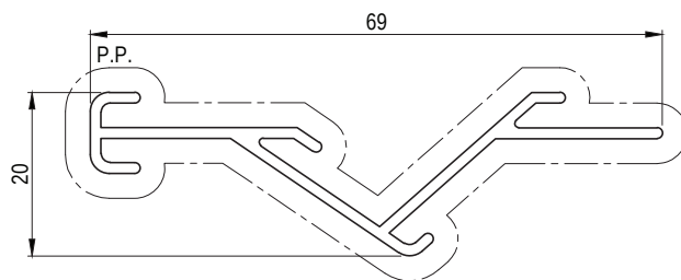
EA1148 62 x 47.5mm BLADE Paint Perimeter: 234mm Anodised Perimeter: 234mm NOT STOCKED
