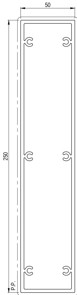
EP19036 50 x 250mm BOX LOUVRE Paint Perimeter: 599mm Anodised Perimeter: 599mm
