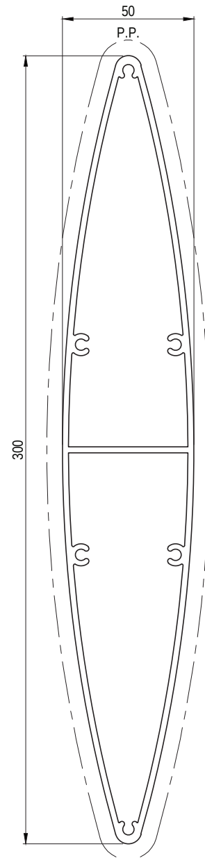
EP11641 300mm ELLIPTICAL BLADE Paint Perimeter: 619mm Anodised Perimeter: 619mm
