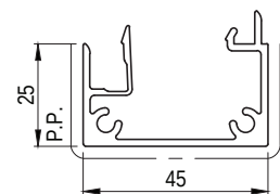
EP14309 45mm BOX LOUVRE END SNAP Paint Perimeter: 197mm Anodised Perimeter: 295mm
