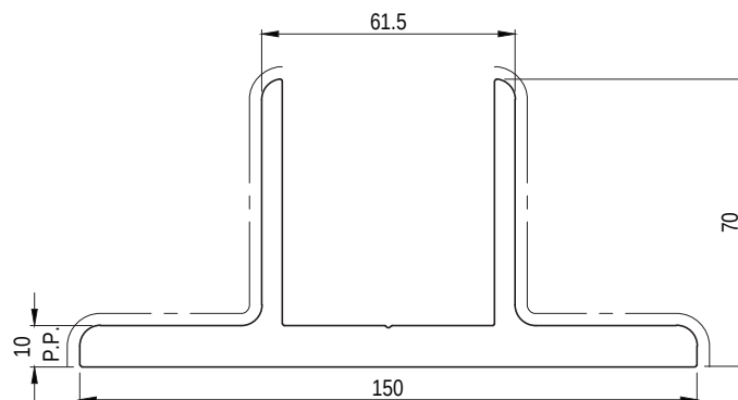
EP15199 50mm BOX LOUVRE BRACKET Paint Perimeter: 364mm Anodised Perimeter: 546mm
