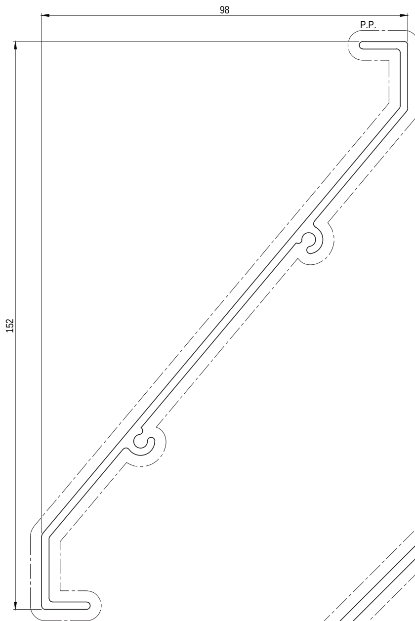
E31090 152 x 98mm BLADE Paint Perimeter: 454mm Anodised Perimeter: 454mm NOT STOCKED
