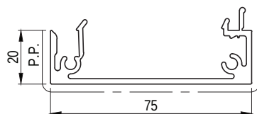
EP15127 75mm BOX LOUVRE END SNAP Paint Perimeter: 232mm Anodised Perimeter: 347mm
