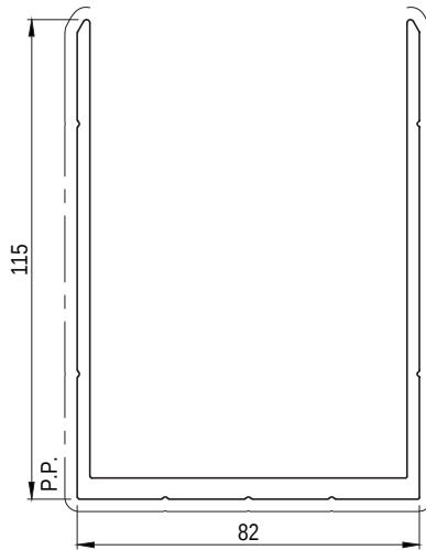
EP17873 75mm BOX LOUVRE CHANNEL Paint Perimeter: 410mm Anodised Perimeter: 613mm
