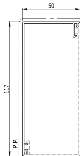
EQ7013 117 x 50mm S/M BOX LOUVRE Paint Perimeter: 165mm Anodised Perimeter: 381mm NOT STOCKED
