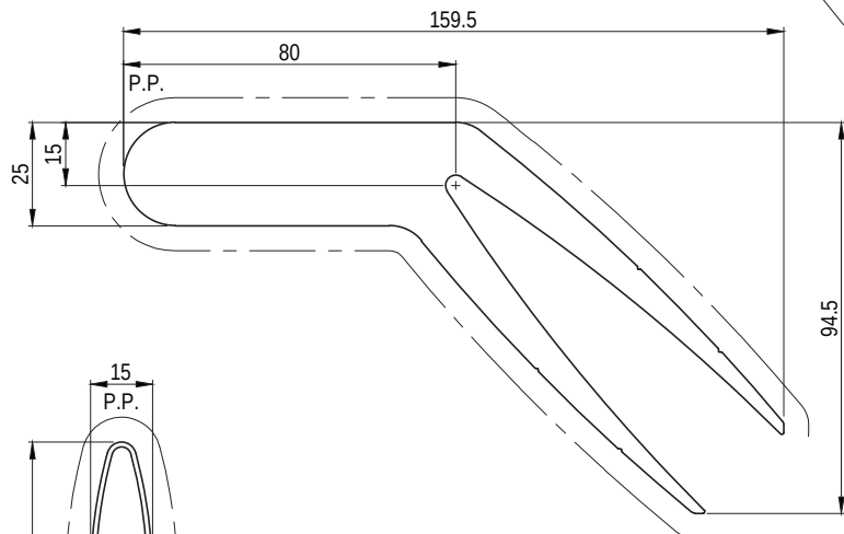
EP9771 200mm LOUVRE BRACKET Paint Perimeter: 378mm Anodised Perimeter: 583mm
