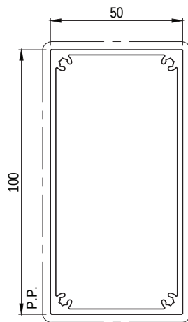
EP16524 50 x 100mm BOX LOUVRE Paint Perimeter: 299mm Anodised Perimeter: 299mm
