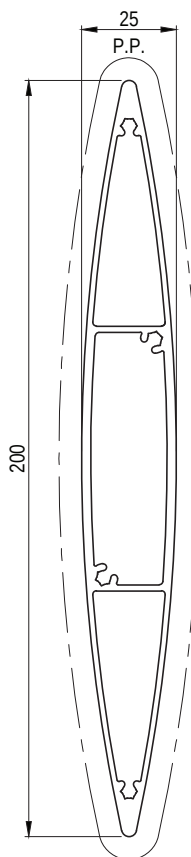
EP9732 200mm ELLIPTICAL BLADE Paint Perimeter: 408mm Anodised Perimeter: 408mm
