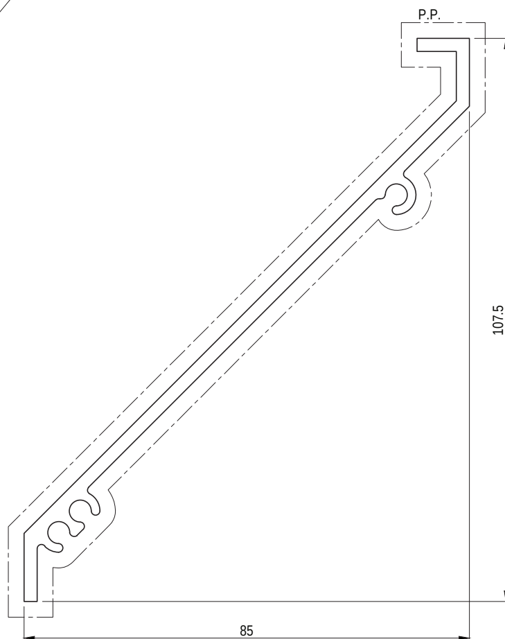
EL1671 107 x 85mm BLADE Paint Perimeter: 346mm Anodised Perimeter: 346mm
