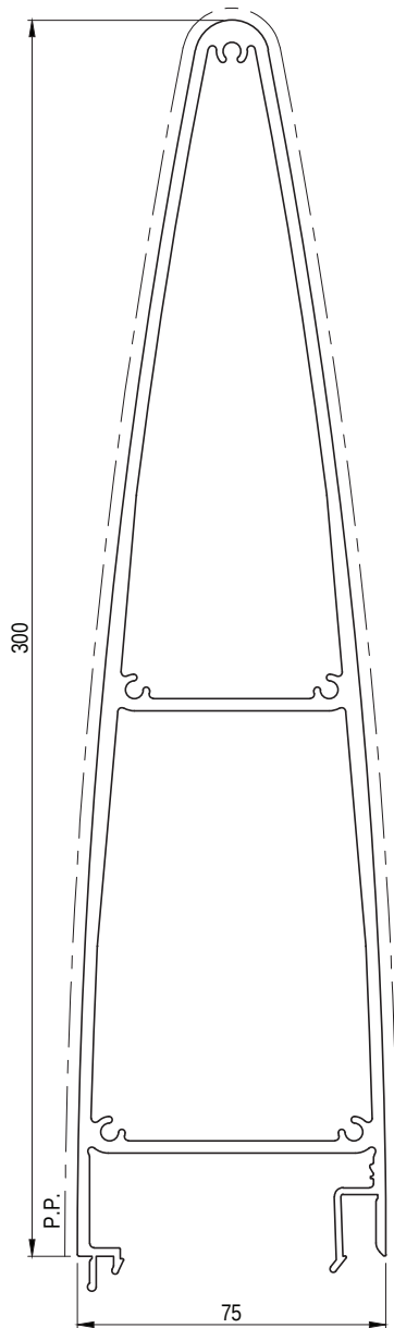
EP15124 75mm BOX LOUVRE BULLNOSE Paint Perimeter: 615mm Anodised Perimeter: 842mm
