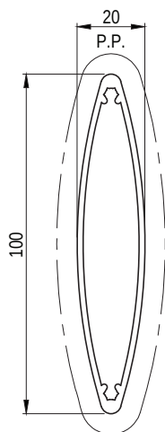
EP7682 100mm ELLIPTICAL BLADE Paint Perimeter: 210mm Anodised Perimeter: 210mm
