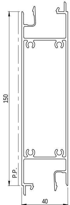
EP13263 40mm INTERMEDIATE BOX LOUVRE Paint Perimeter: 432mm Anodised Perimeter: 647mm
