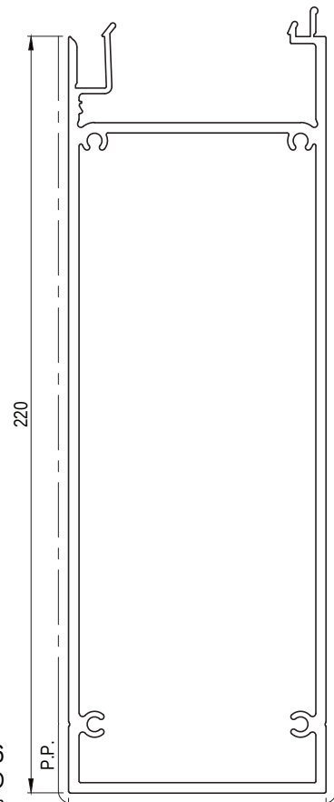
EP15126 75mm BOX LOUVRE END Paint Perimeter: 406mm
