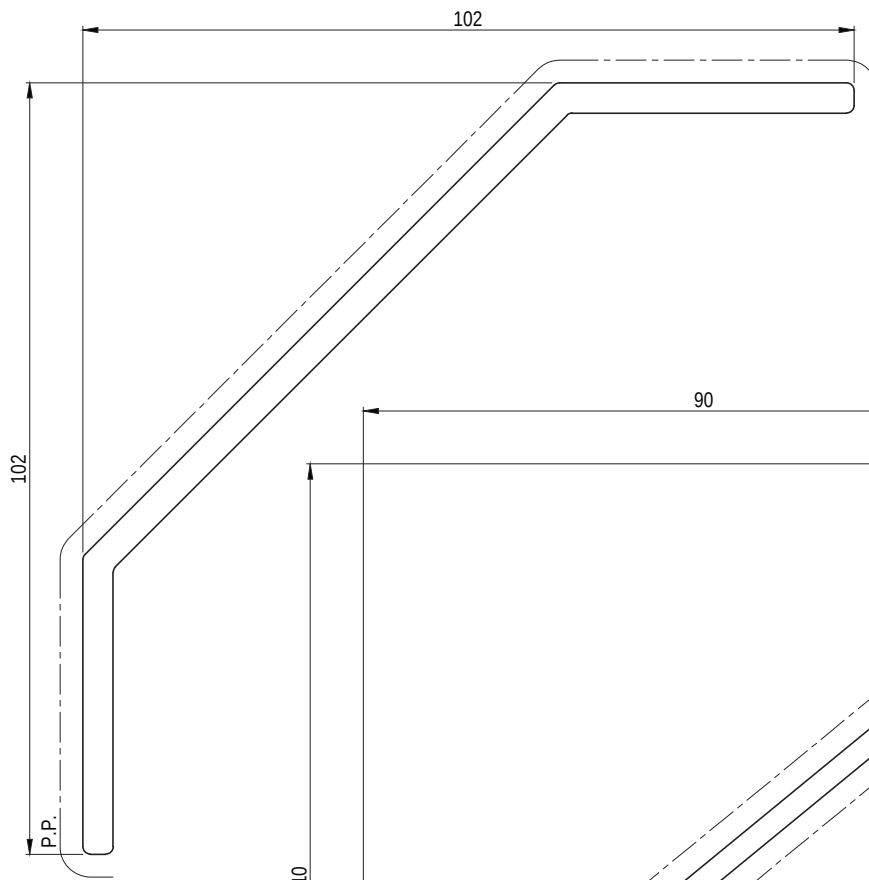
E32590 102mm BLADE Paint Perimeter: 176mm Anodised Perimeter: 334mm NOT STOCKED
