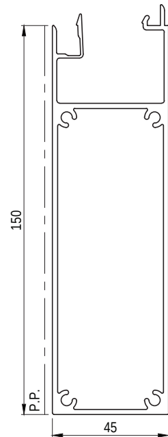
EP14308 45mm BOX LOUVRE 150mm END Paint Perimeter: 456mm Anodised Perimeter: 684mm
