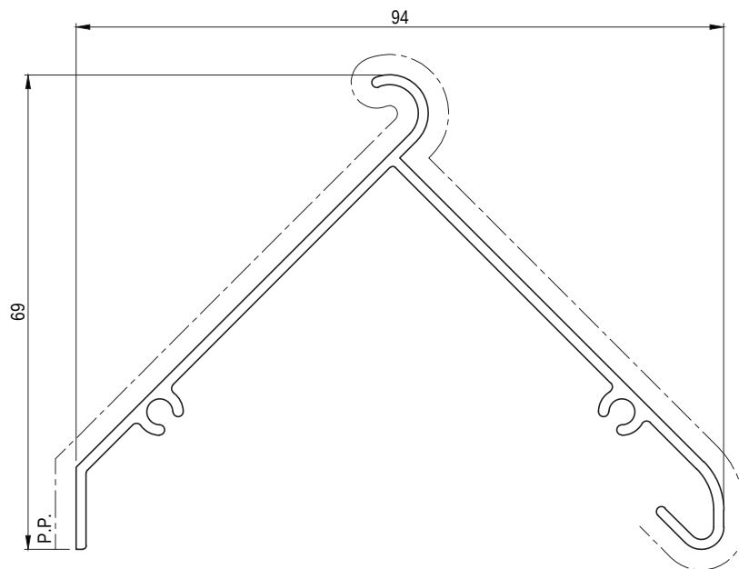
E53522 69 x 94mm DOUBLE SIDED LOUVRE Paint Perimeter: 202mm Anodised Perimeter: 388mm NOT STOCKED
