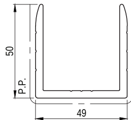
EP14150 40mm BOX LOUVRE CHANNEL Paint Perimeter: 191mm Anodised Perimeter: 286mm
