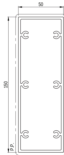
EP19038 50 x 150mm BOX LOUVRE Paint Perimeter: 399mm Anodised Perimeter: 399mm
