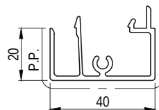
EP13264 40mm BOX LOUVRE END SNAP Paint Perimeter: 179mm Anodised Perimeter: 268mm
