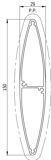
EP9282 150mm ELLIPTICAL BLADE Paint Perimeter: 312mm Anodised Perimeter: 312mm
