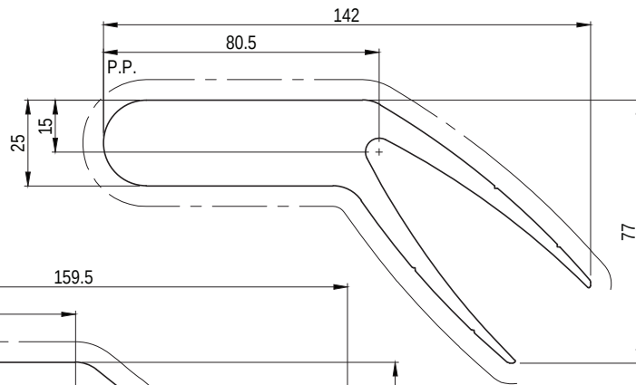
EP9799 150mm LOUVRE BRACKET Paint Perimeter: 323mm Anodised Perimeter: 480mm
