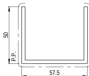
EP13476 50mm BOX LOUVRE CHANNEL Paint Perimeter: 206mm Anodised Perimeter: 308mm
