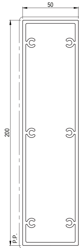
EP19037 50 x 200mm BOX LOUVRE Paint Perimeter: 499mm Anodised Perimeter: 499mm
