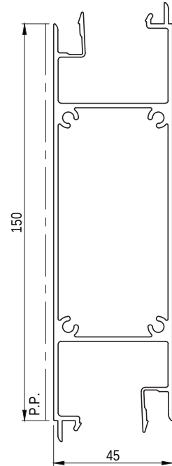
EP13691 45mm INTERMEDIATE BOX LOUVRE Paint Perimeter: 456mm Anodised Perimeter: 684mm
