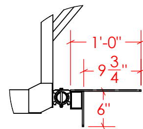
DETAIL A SEAWALL ATTACHMENT
