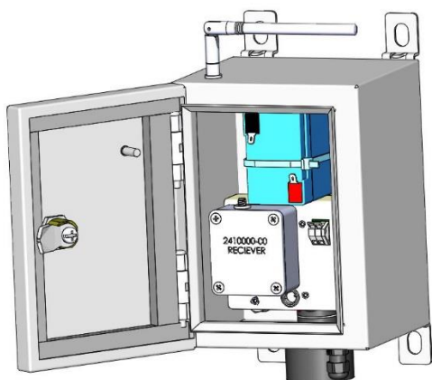
Stainless (SS) or Painted Steel (PS) Enclosure
