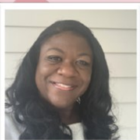
Taneka Williams
