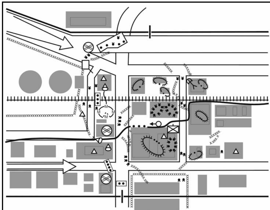
Figure 5-21. Urban strongpoint.
