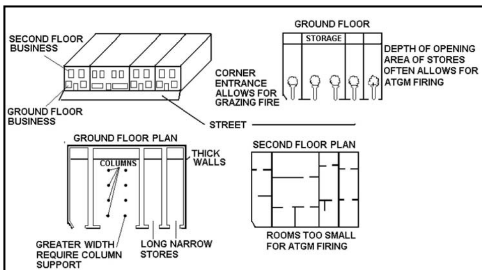
Figure 2-18. Brick structures.
