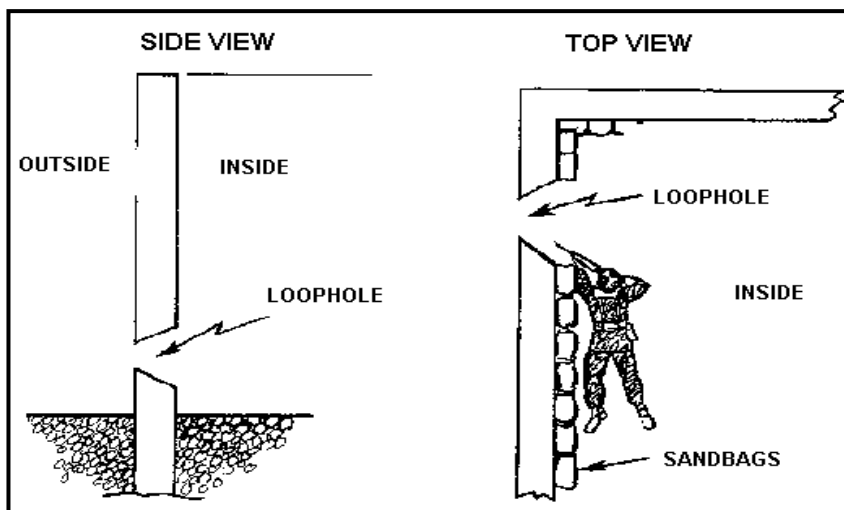
Figure 3-48. Prepared loophole.
