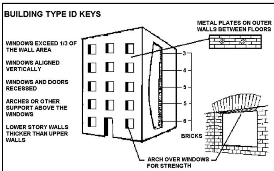
Figure 2-17. Brick buildings.
