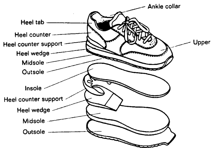
Figure 4-1. Parts of a Running Shoe
