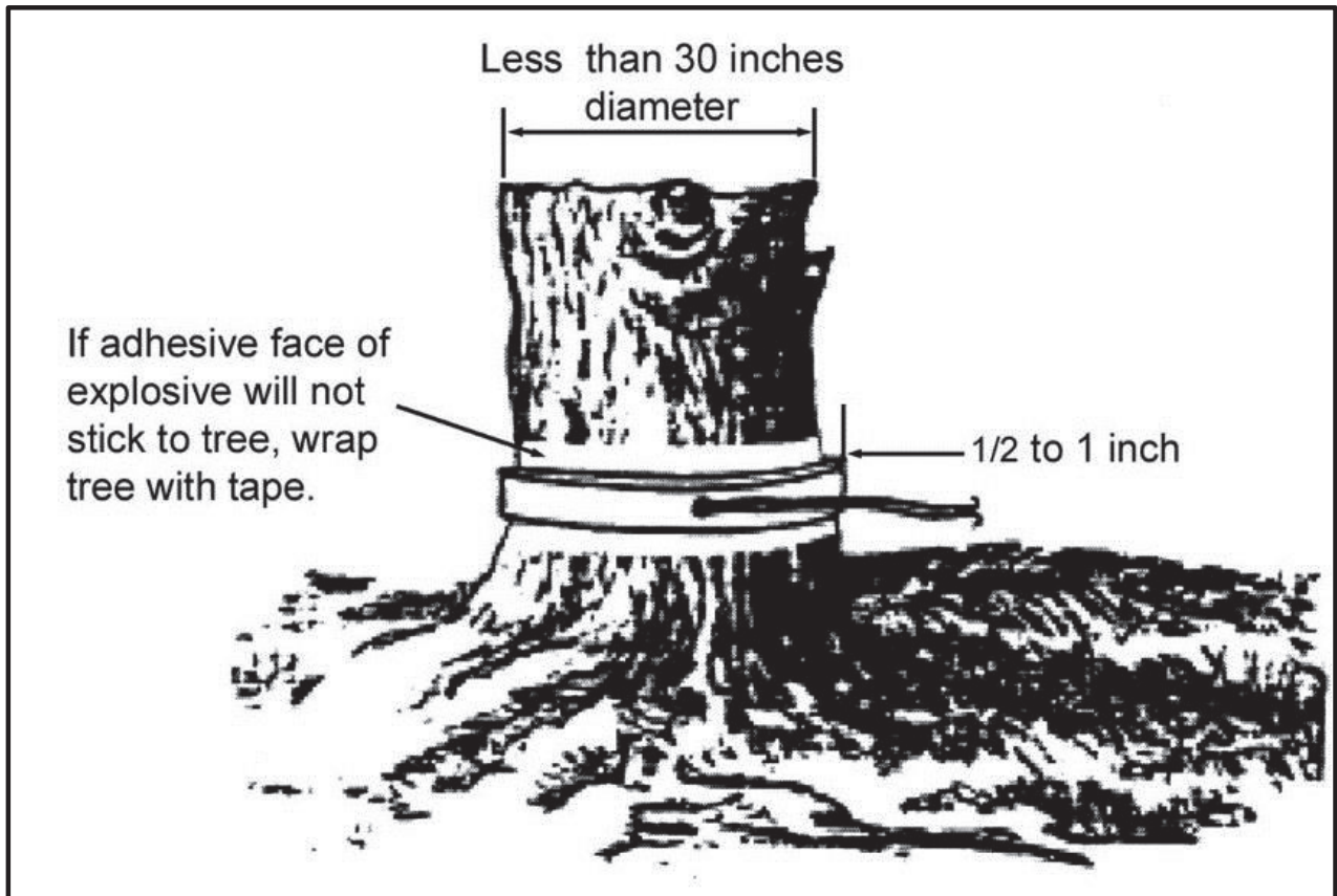
Figure 5-11. Timber-cutting ring charge
