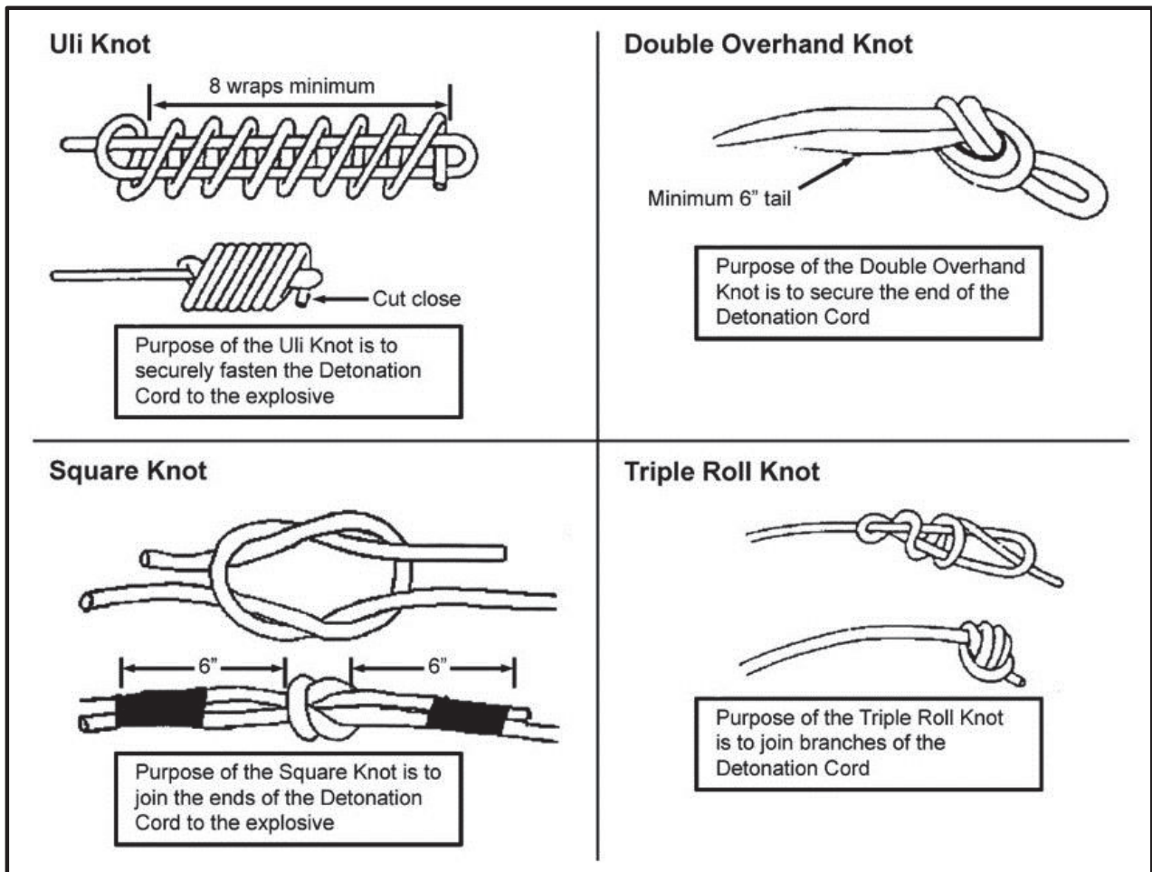
Figure 5-5. Various joining knots used in demolitions
