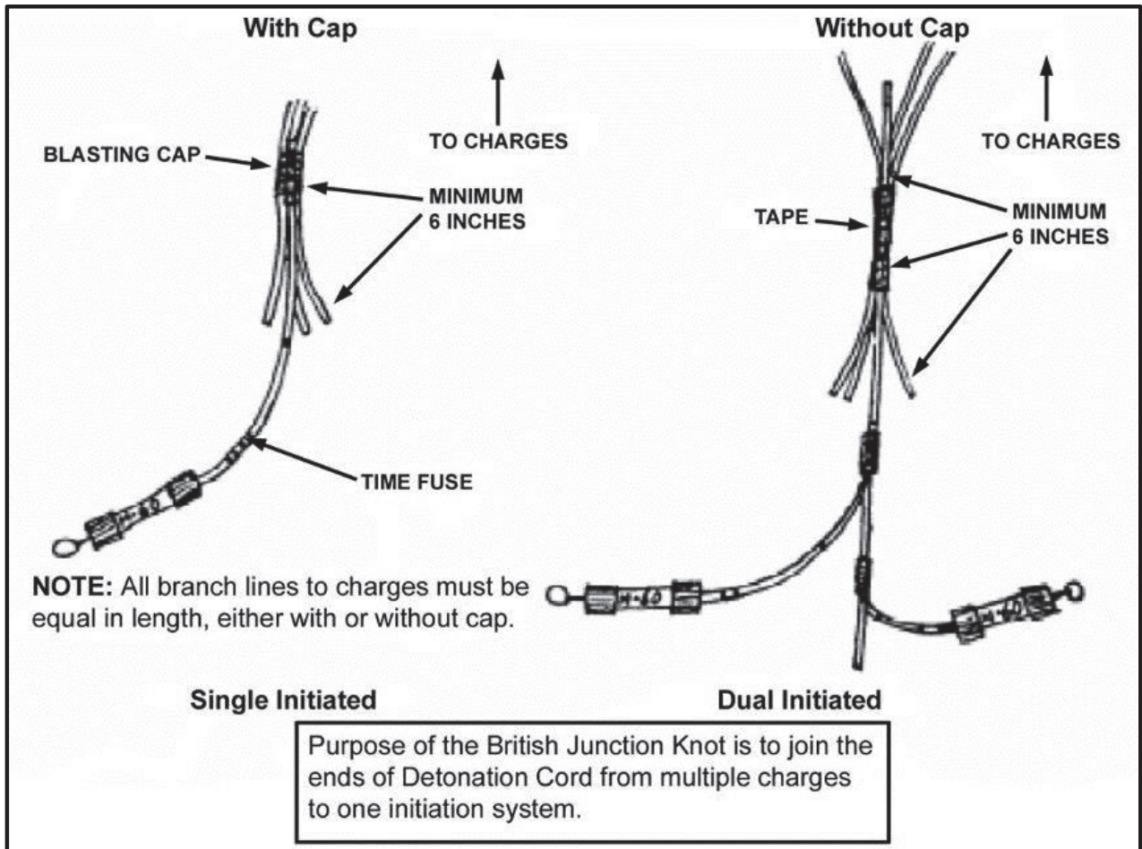
Figure 5-6. British junction knot
