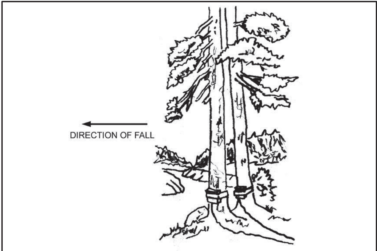
Figure 5-12. Timber-cutting charge (external)
