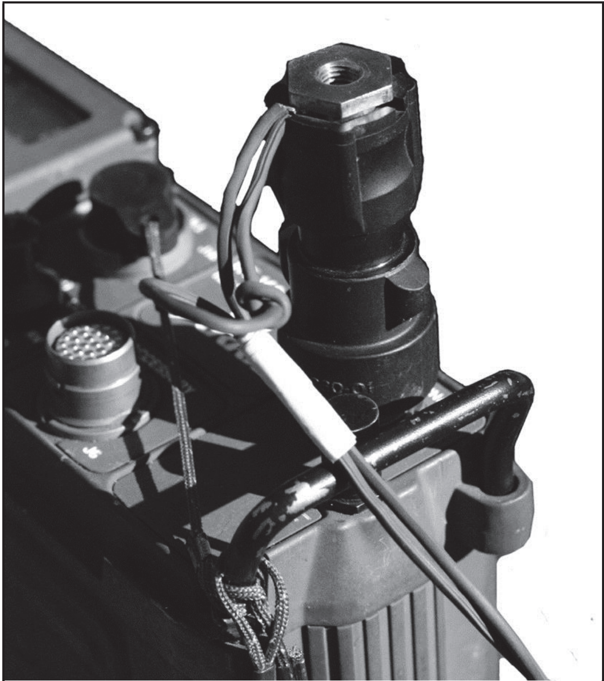
Figure 4-2. Antenna base
