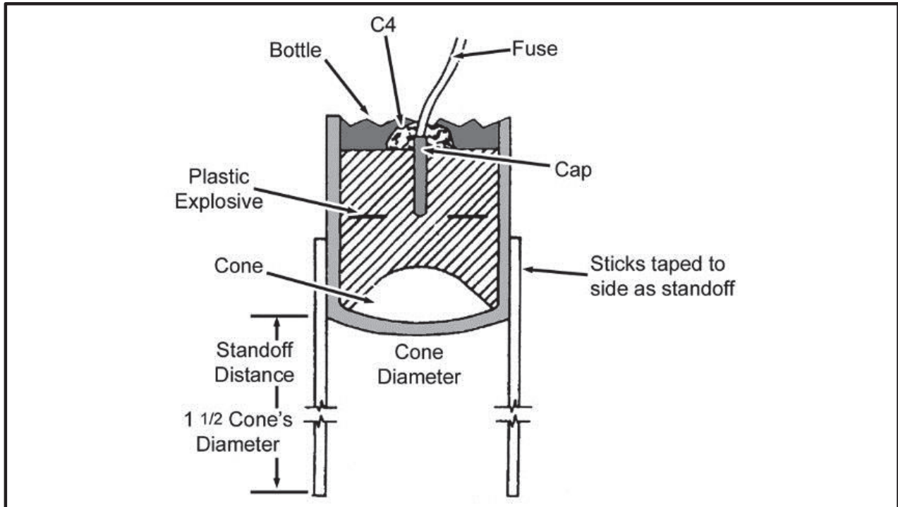
Figure 5-2. Improved shape charge
