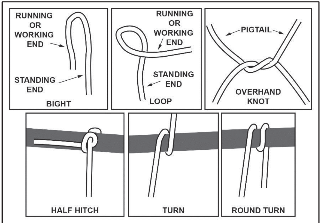
Figure 9-5. Rope terminology
