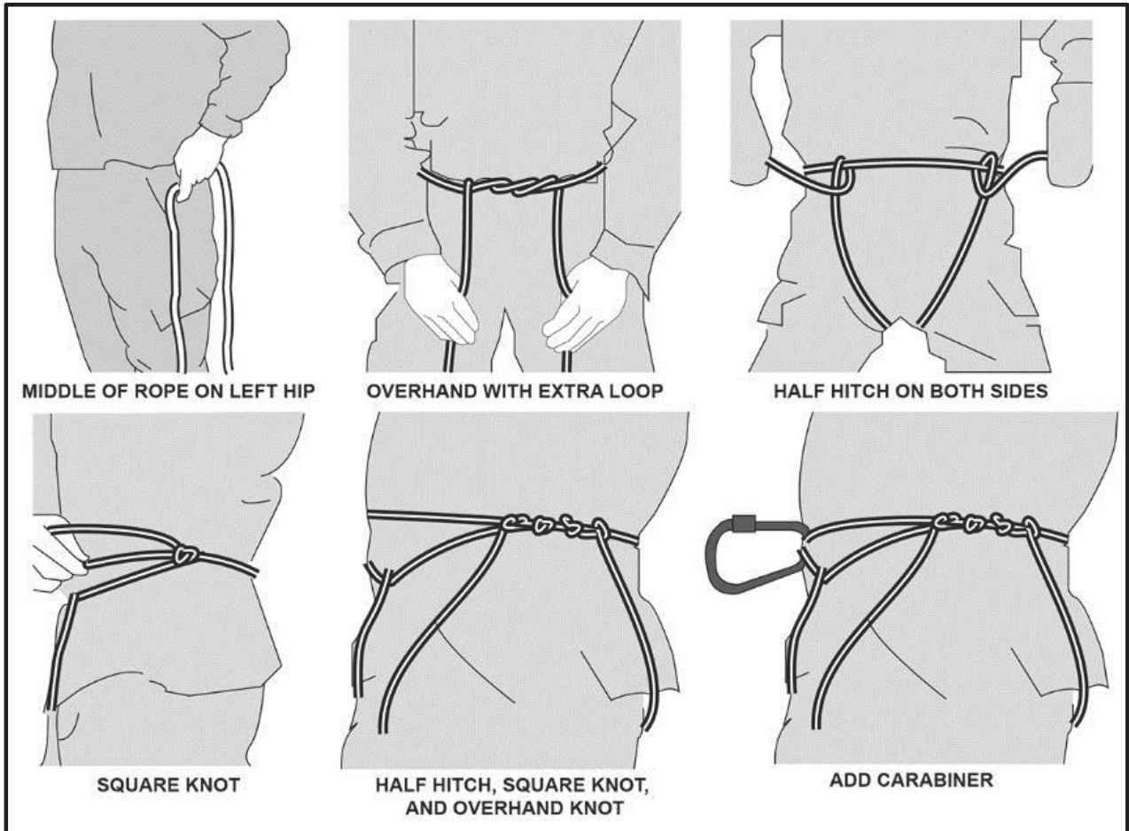
Figure 9-11. Rappel seat
