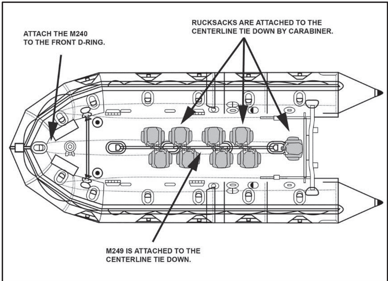
Figure 12-5. Equipment rigging
