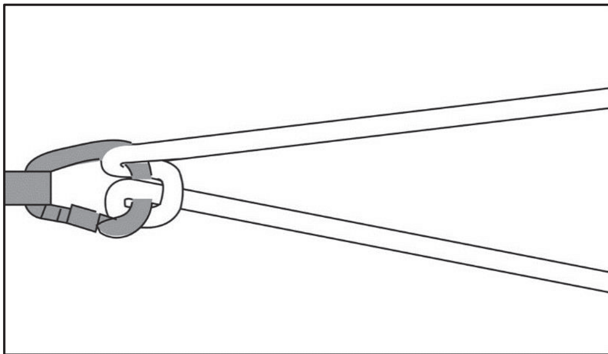
Figure 9-14. Munter hitch
