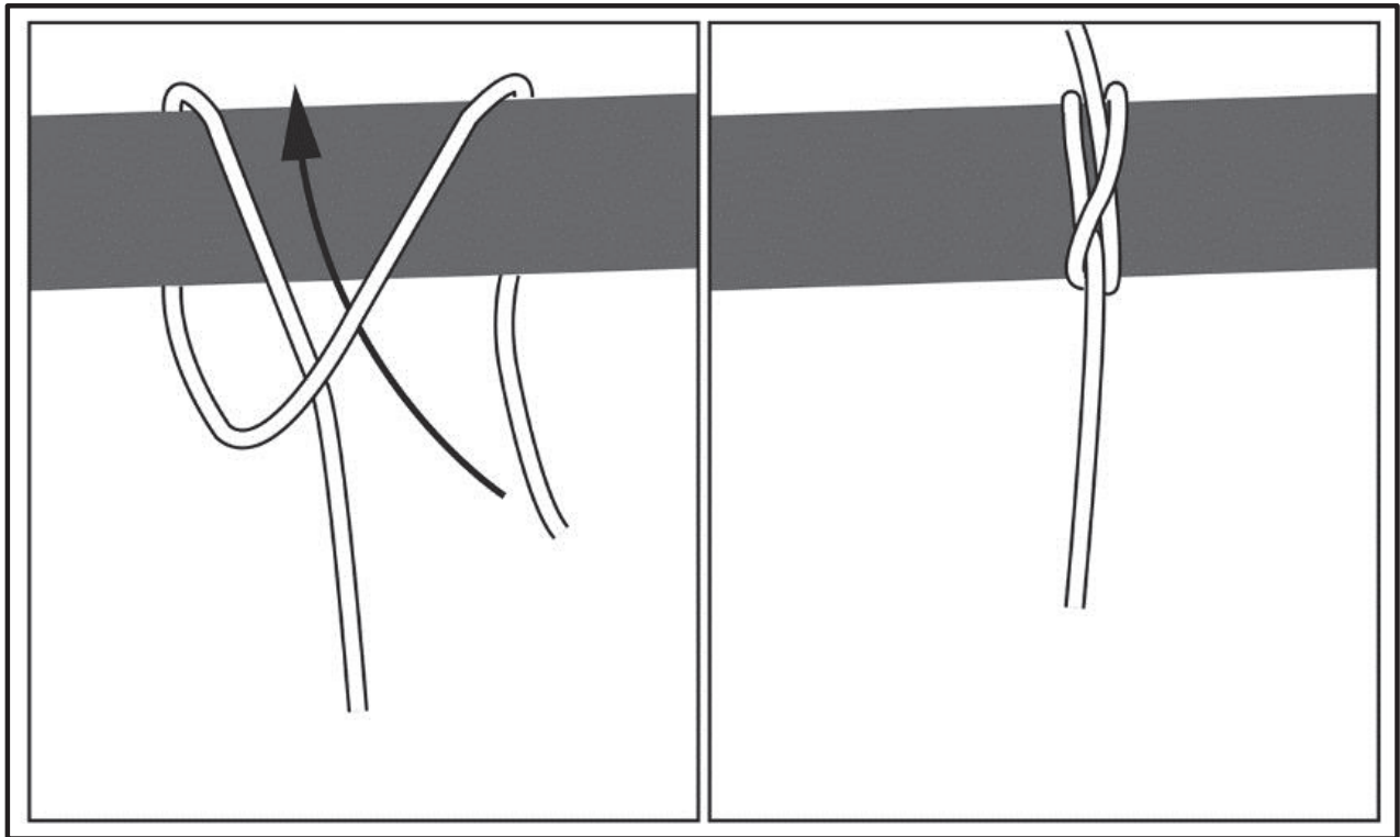
Figure 9-9. End-of-the-rope clove hitch
