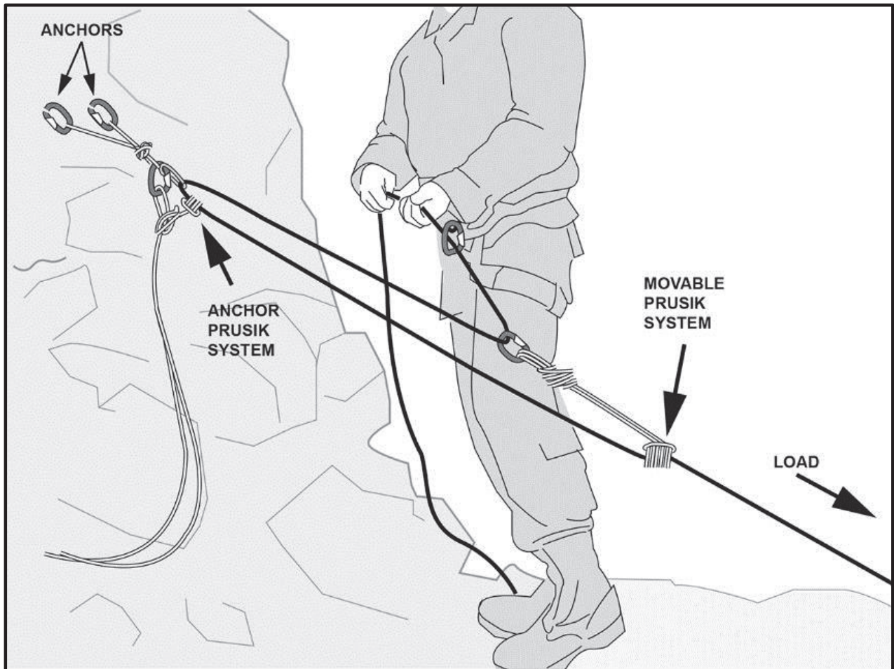
Figure 9-24. Z-Pulley system
