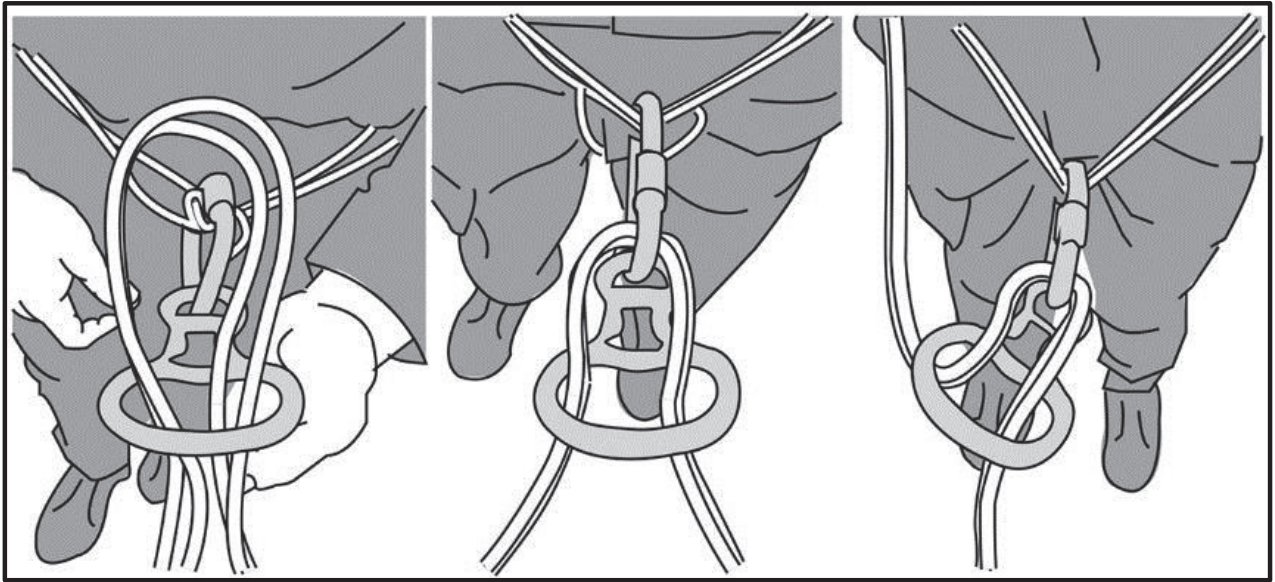
Figure 9-27. Figure-eight descender
