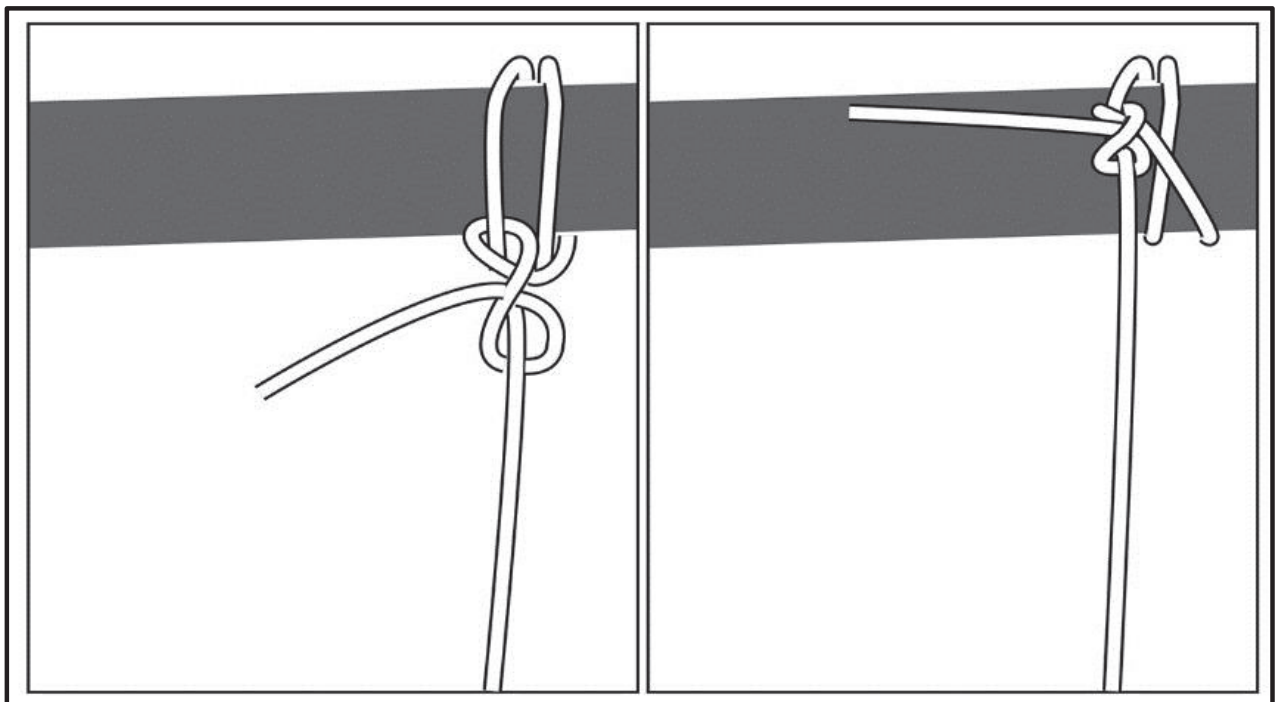
Figure 9-7. Round turn with two half hitches
