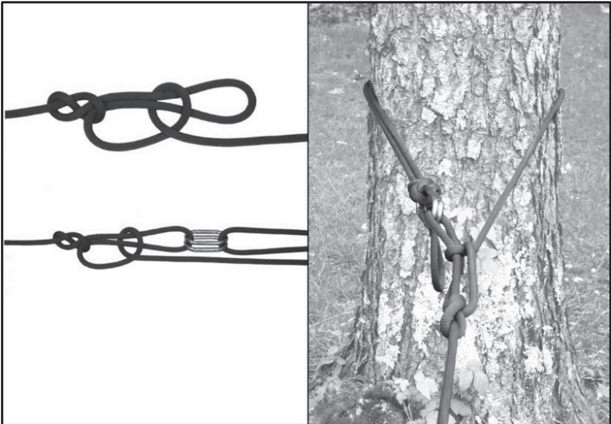
Figure 12-2. Transport-tightening system
