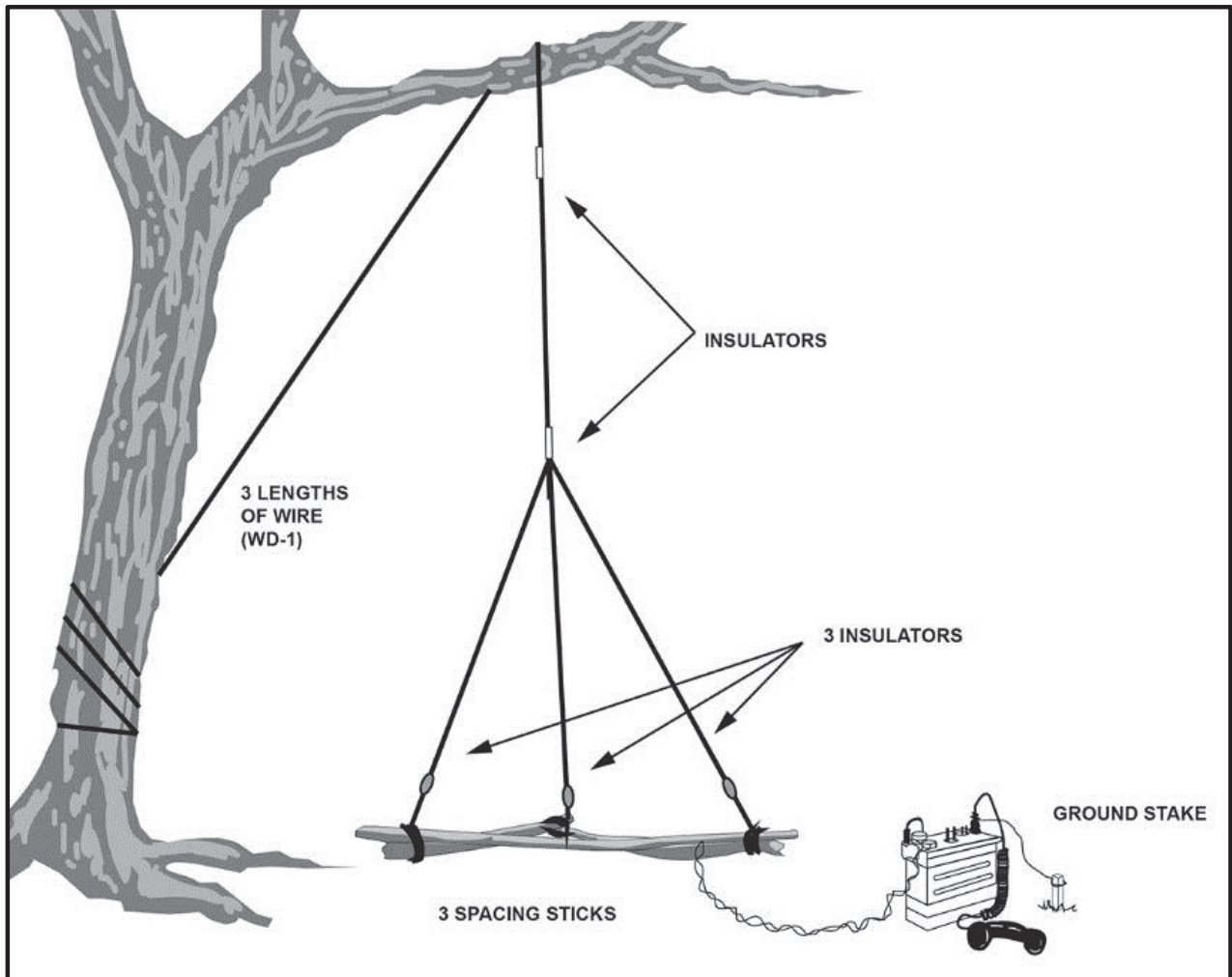
Figure 4-3. Completed expedient 292-type antenna
