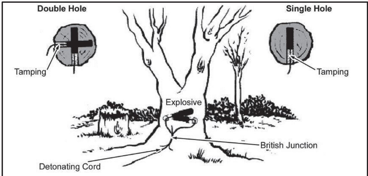
Figure 5-14. Timber-cutting charge (internal)
