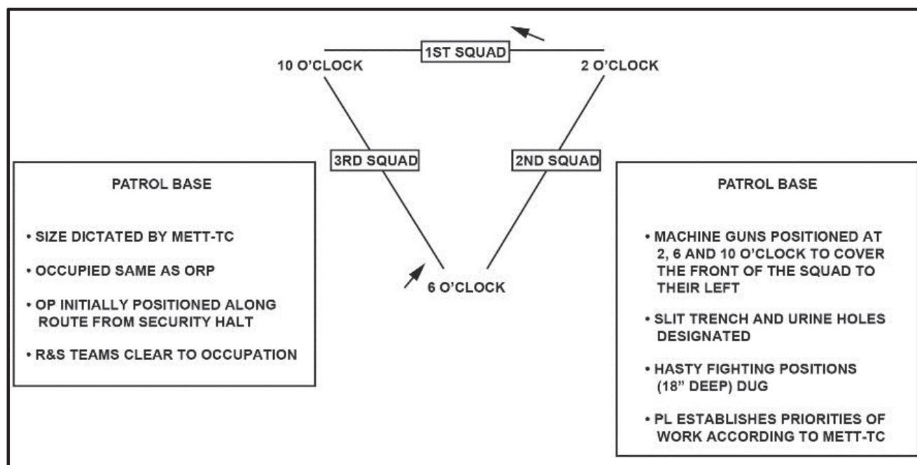
Figure 7-7. Patrol base
