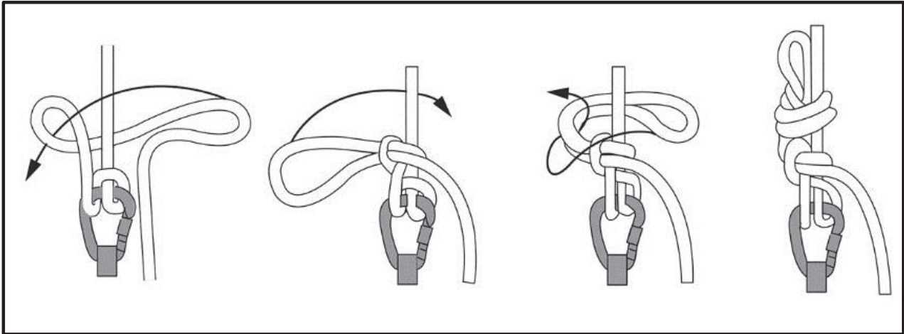
Figure 9-15. Munter mule knot
