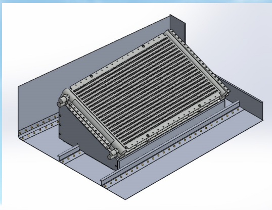
Tailcone mounted condenser coils use out of sight belly mounted louver pan-
