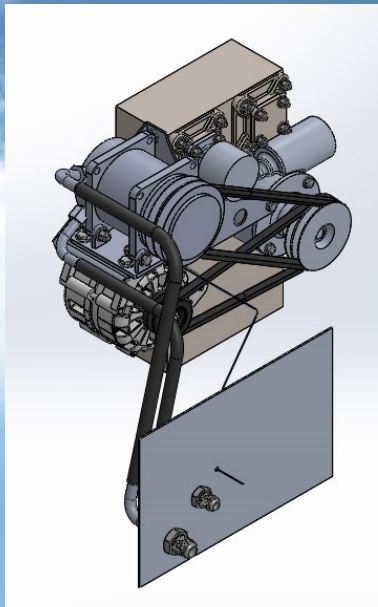
Engine driven compressor mounts on accessory case with a low mounted alternator location.
