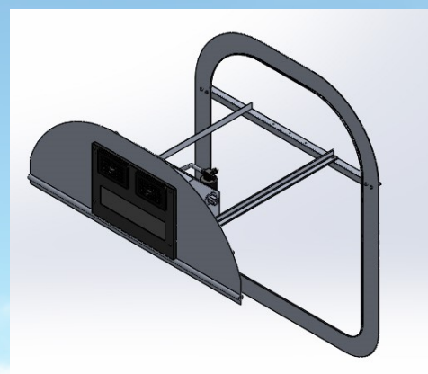
Evaporator unit mounts on baggage compartment bulkhead and includes directional louver vents.
