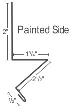
⑧ Peak Sheet
