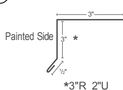
㉑ Short Eave Trim
