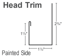
⑯ Head Trim
