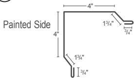
⑫ Outside Corner
