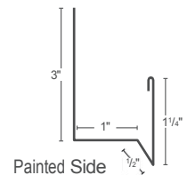
⑪ Sculptured Rake
