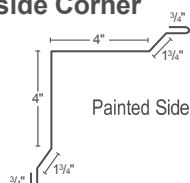
⑬ Inside Corner
