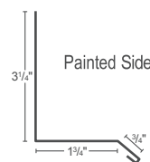
⑱ Base Trim
