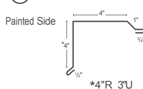
㉒ Residential Rake
