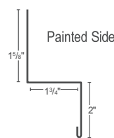
⑥ Wainscott Trim
