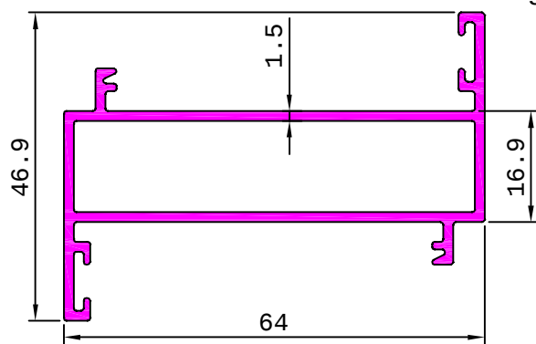
S5487 0.887 kg/m
