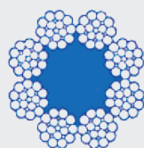
8x21 Filler Fiber Core
