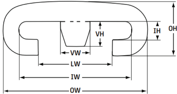
Nominal Dimensions (mm, +/- 0.5mm)
