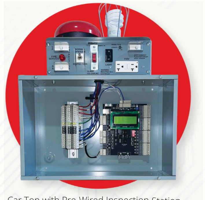
Car Top with Pre-Wired Inspection Station
