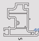
703810 61mm Flush Sash
