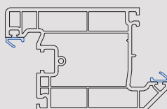
705510 110mm Door Sash Open In
