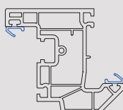
703509 79mm Tilt & Turn Sash
