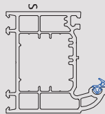
101161 70mm Outerframe
