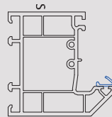
701502 72mm Outerframe
