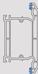
702152 116mm Patio Midrail Bevelled
