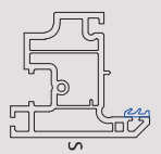
703810 61mm Flush Sash
