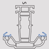
702533 70mm T Transom & French Mullion
