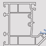
701502 72mm Outerframe
