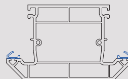
702505 116mm Midrail
