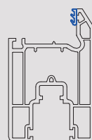
705151 90mm Patio Sash Bevelled
