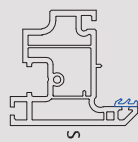
703810 61mm Flush Sash
