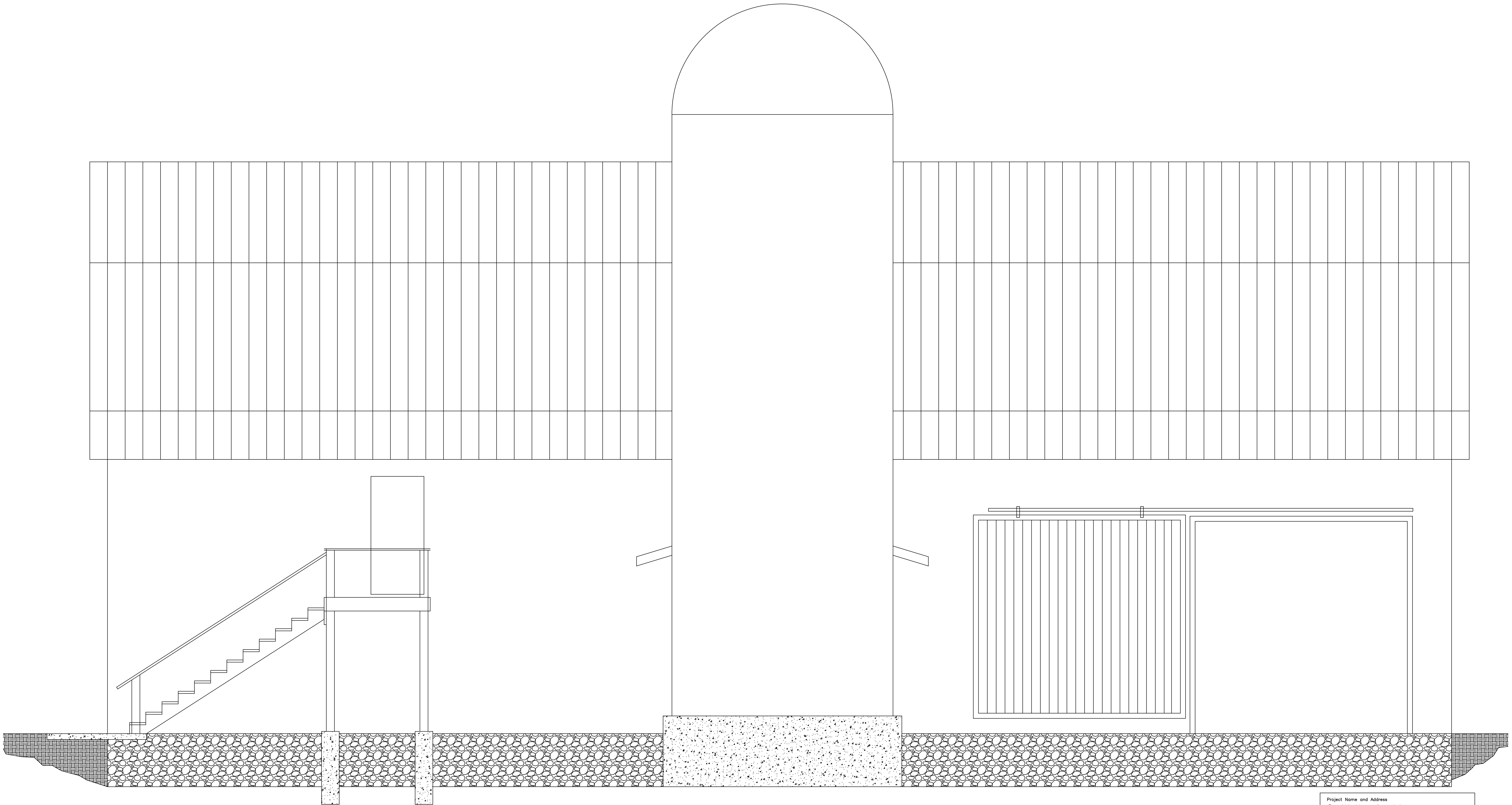
East Elevation
