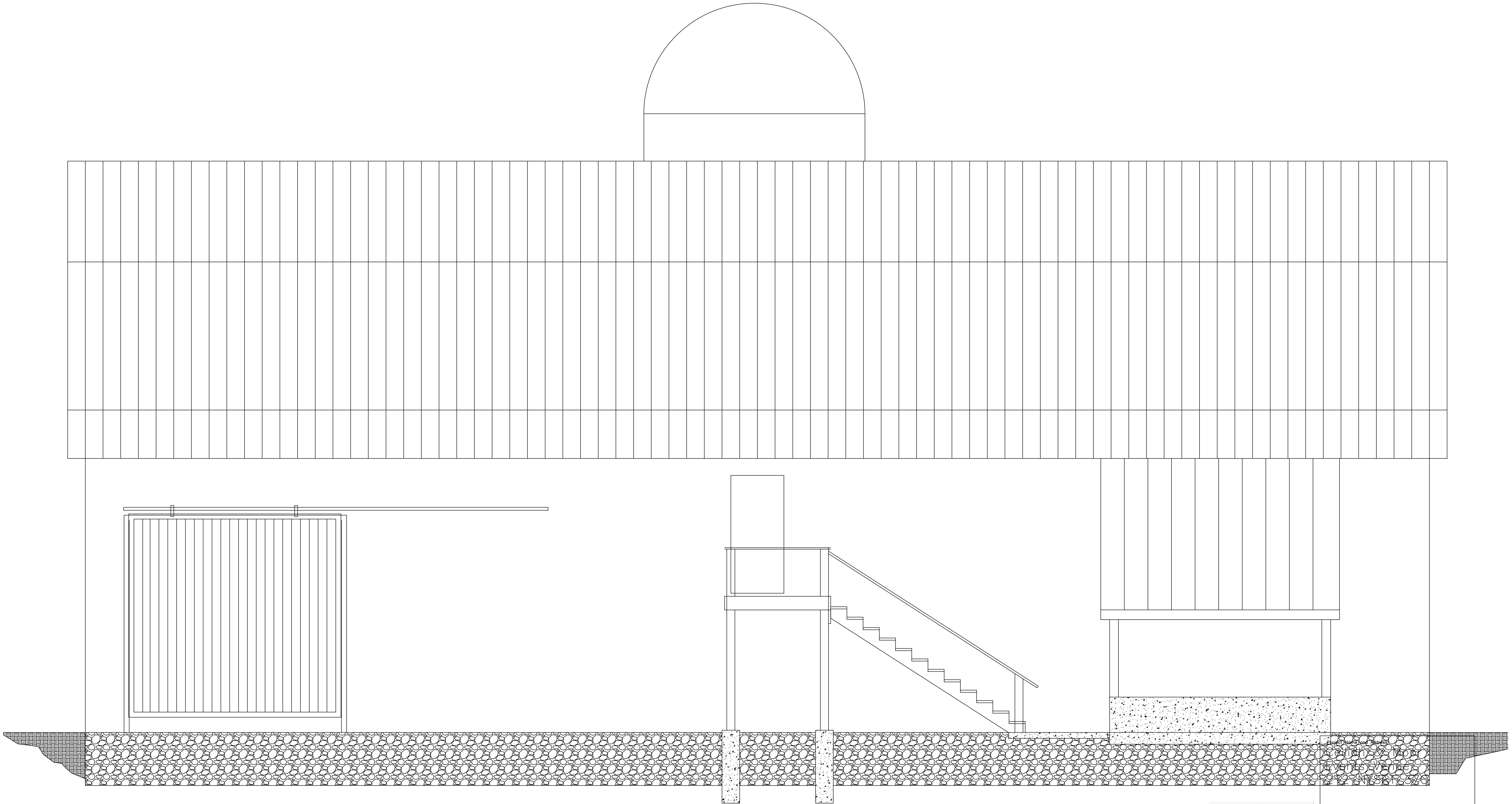
West Elevation
