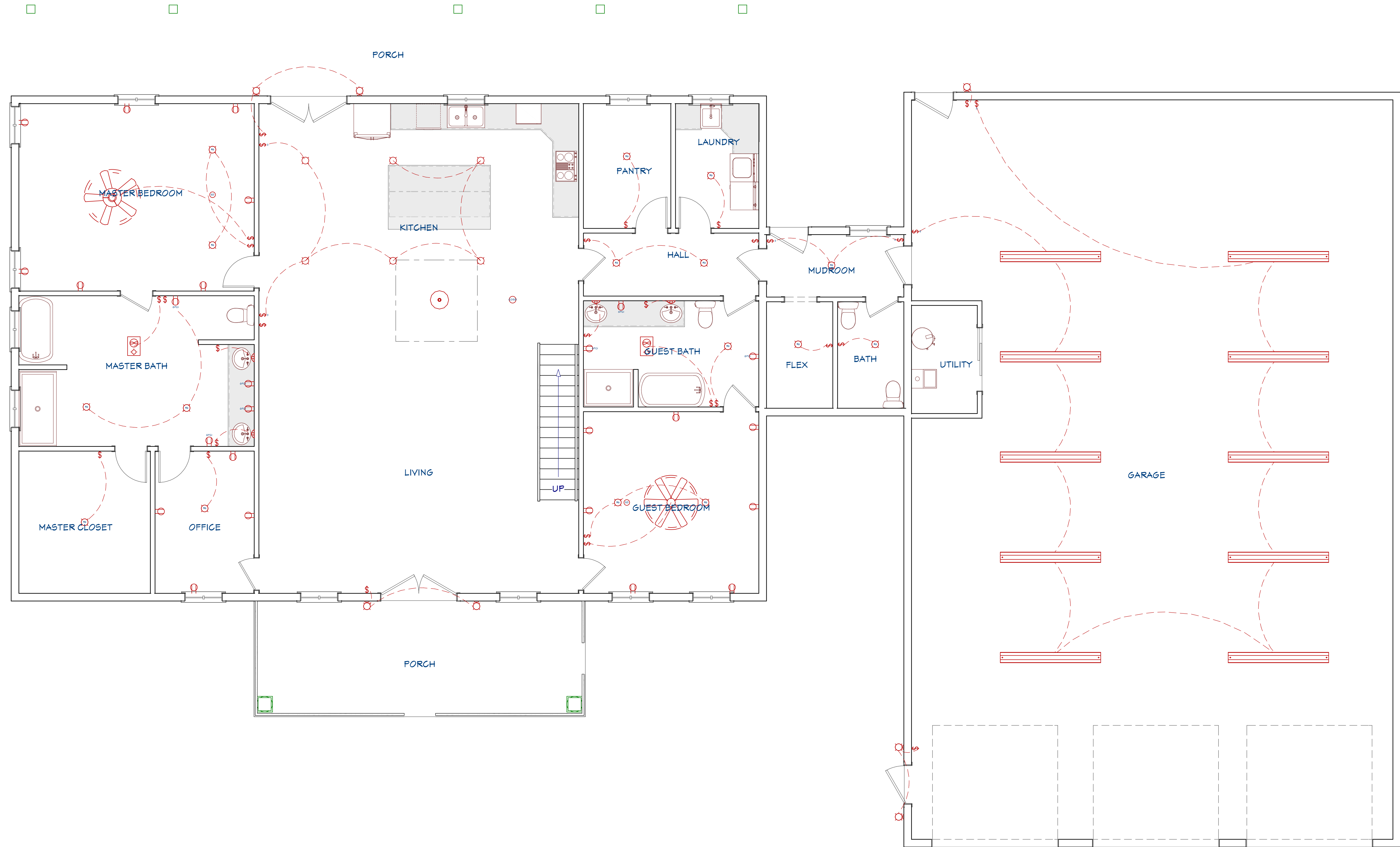
1ST FLOOR ELECTRICAL PLAN
