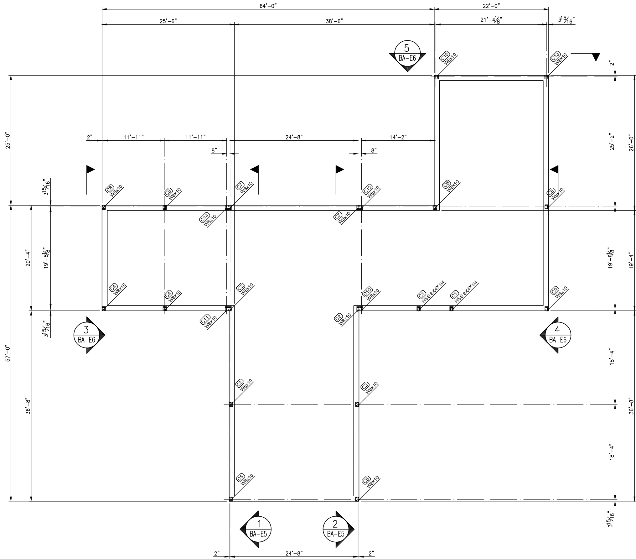
LUC BAUDOUIN – COLUMN LAYOUT SCALE: 3/16"=1'-0"
