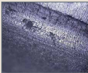
Identification of corrosion damage (microdestructions).
