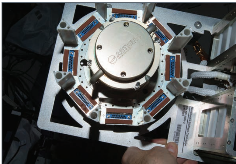
View of Nanoracks Astrium Centrifuge during installation and performance check during Expedition 38 (ISS038E008547).
