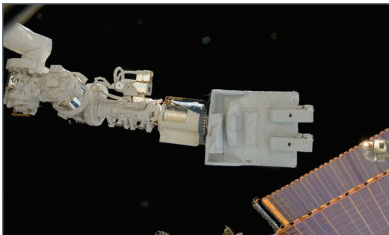
View of the JEMRMS in front of the JEM Airlock (JEMAL) during J-SSOD operations (ISS033E009897).
