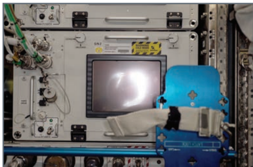
View of the SABL power, data and thermal connections in the rack located in the U.S Laboratory (ISS046E046608).
