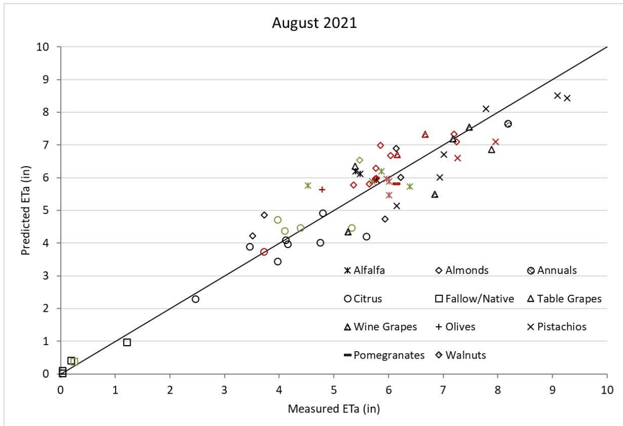
FIGURE 3. MEASURED VERSUS PREDICTED ET a FOR THE MONTH. SYMBOL COLORS REPRESENT THE STATION TYPES (BLACK = FULL, GREEN = WATER IQ (WIQ), RED = TULE TECH)
