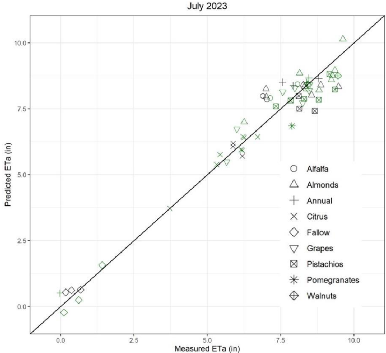
FIGURE 1. MEASURED VERSUS PREDICTED ET A FOR THE MONTH. SYMBOL COLORS REPRESENT THE STATION TYPES (BLACK = FULL, GREEN = WATER IQ (WIQ))
