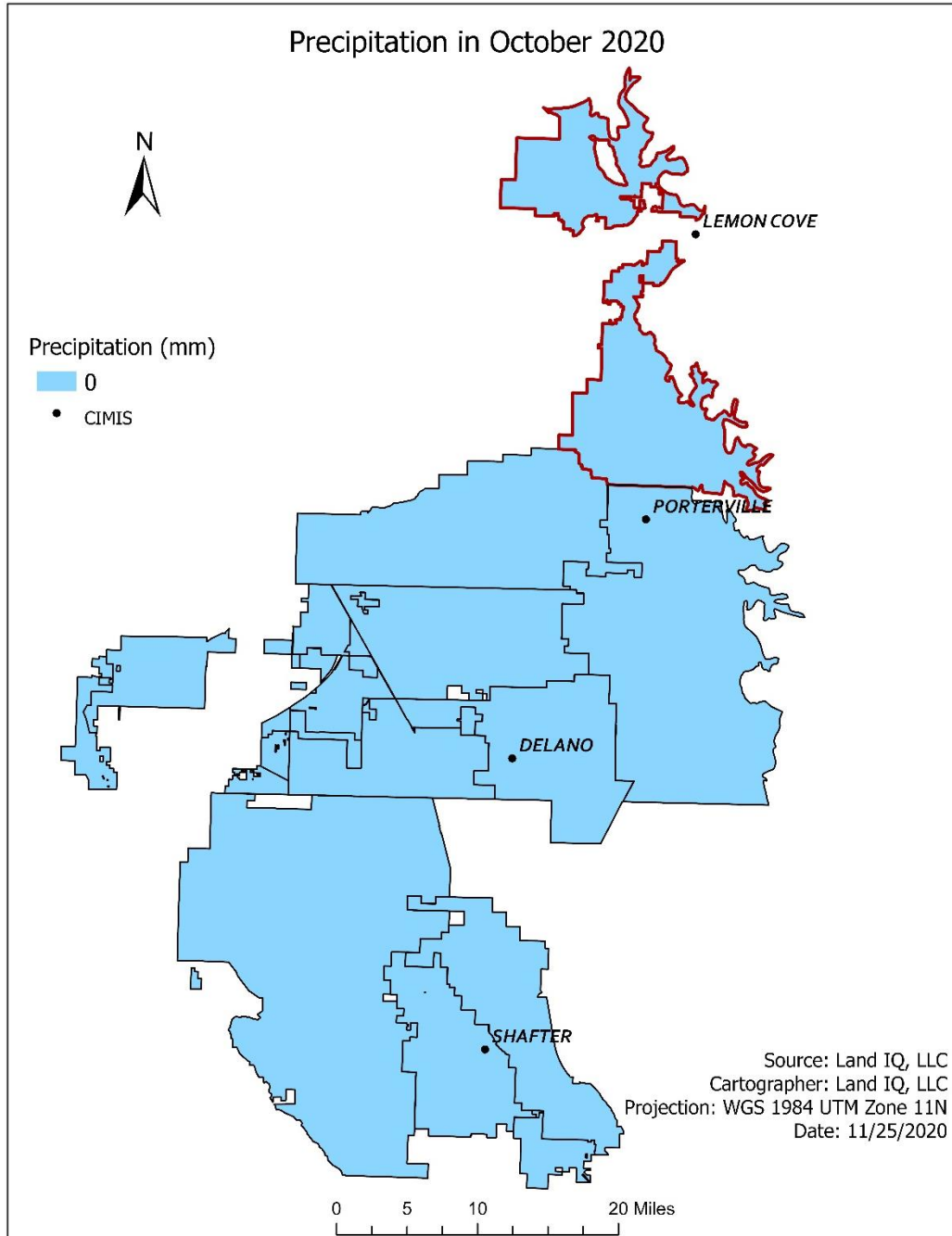
FIGURE 2. PRECIPITATION DURING OCTOBER WITHIN THE ENTIRE ANALYSIS AREA
