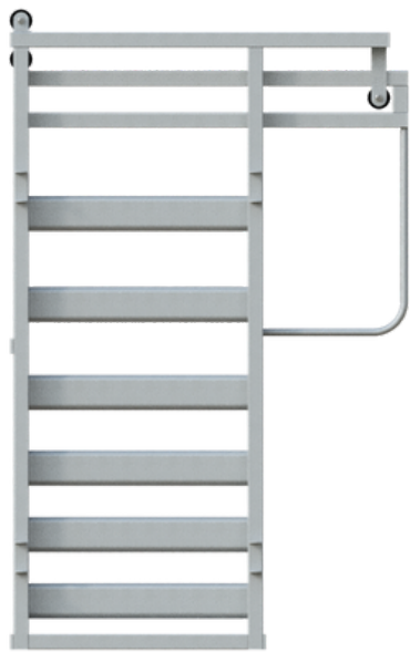
HDCSG1 - Heavy Duty Sliding Gate
