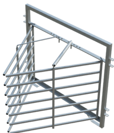
Portable Goat Trap GT1 - 1.7m x 1.35m
