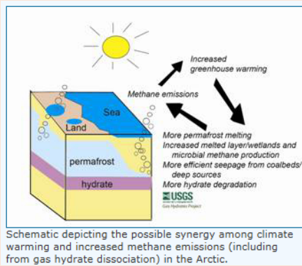
Figure 16.23 Thawing of permafrost and release of carbon dioxide and methane.
