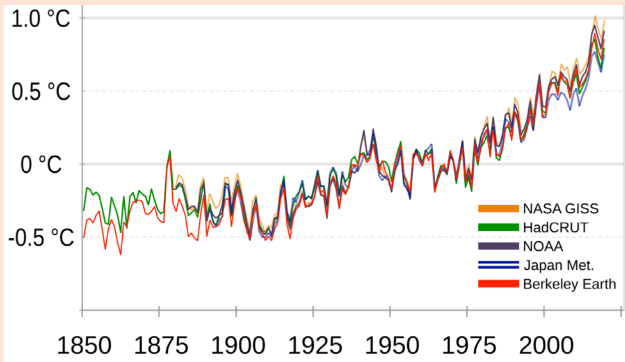
Figure 16.3 Global average temperature change since the beginning of the industrial period.
