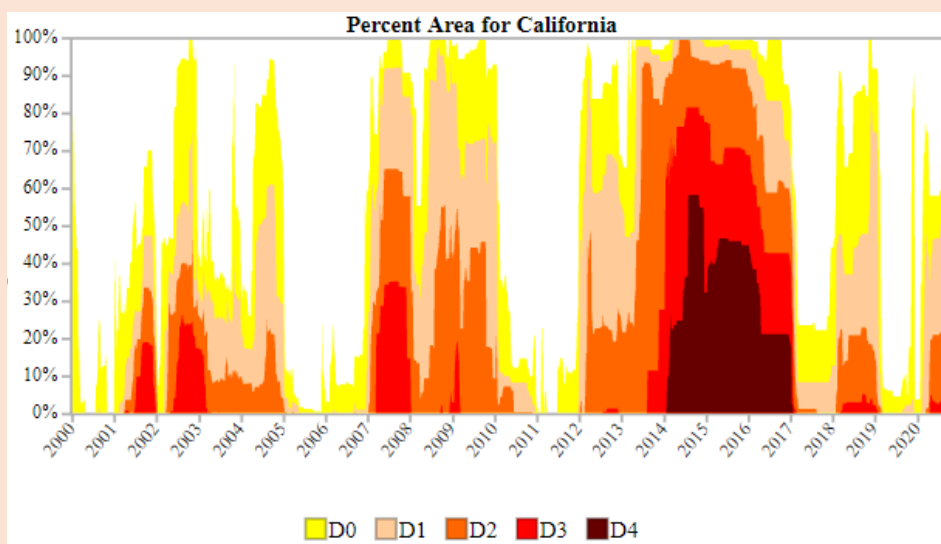
Figure 16.39 Droughts in California since 2000.
