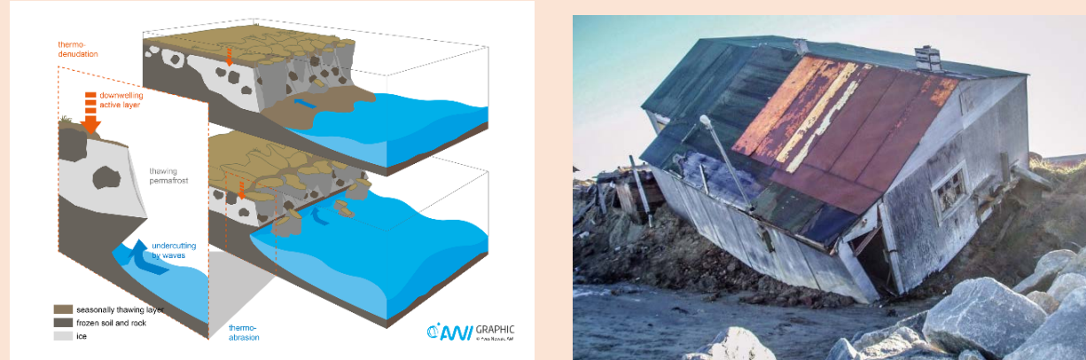
Figure 16.20 Coastal erosion due to permafrost melt.
