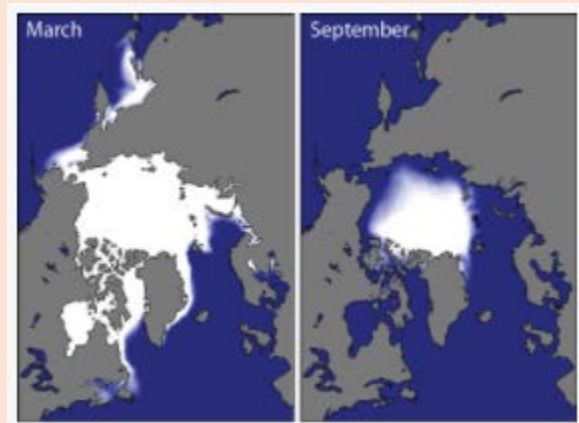
Figure 16.11 Satellite images of Arctic illustrating how sea cover changes from March to September. https://nsidc.org/cryosphere/sotc/sea_ice.html
