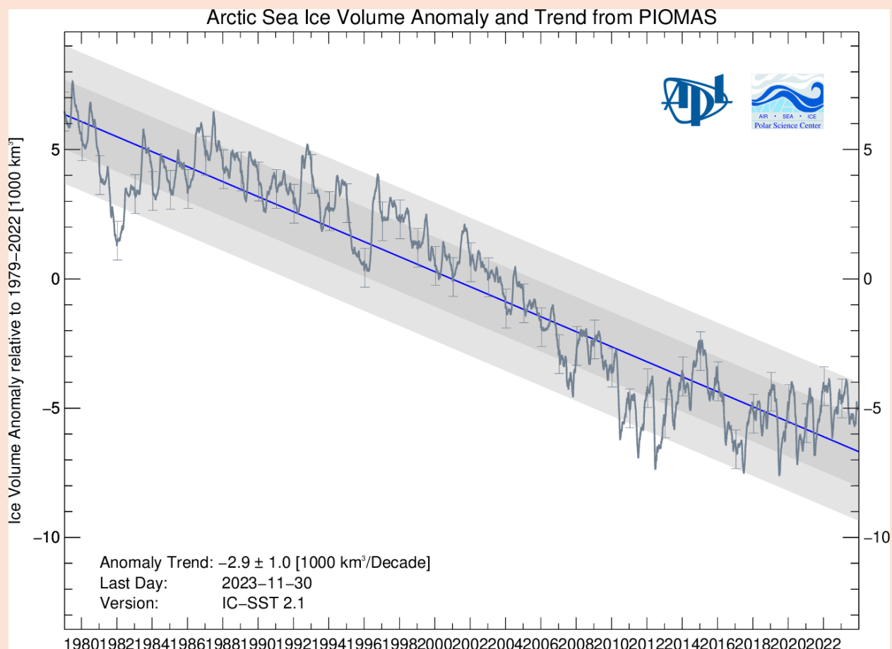
Figure 16.15 Arctic Sea ice volume from analysis by Polar Science Center.
