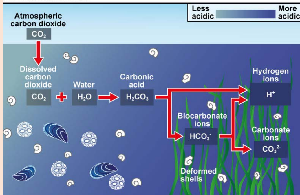
Figure 16.6 Ocean acidification.
