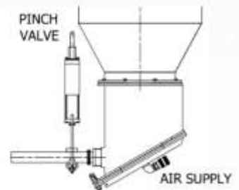
Air Packer
