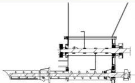
Screw Packer
