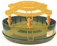
12", 20" & 24" Polylok Riser Safety Screen
