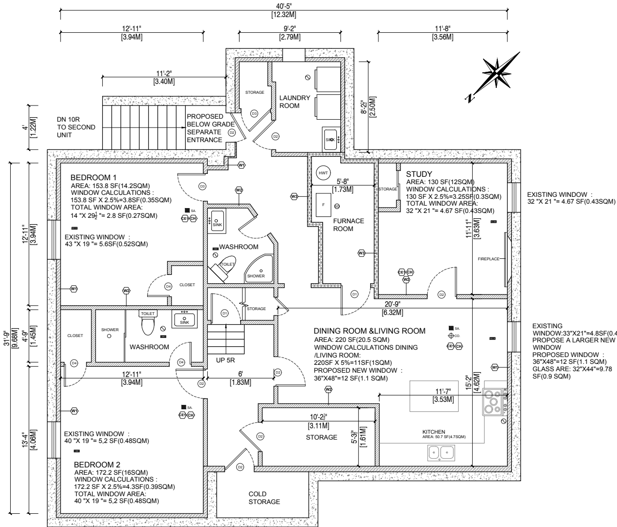
BASEMENT FLOOR PLAN 1:100 BASEMENT TOTAL AREA:1040SF(96.6SQM)
