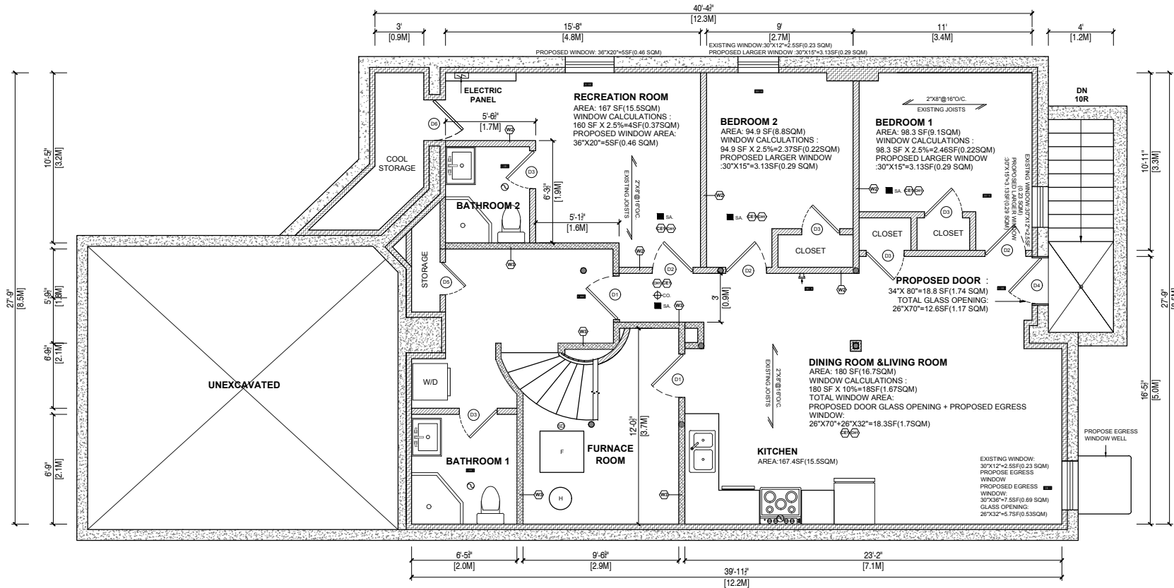
PROPOSED BASEMENT FLOOR PLAN 1:100 PROPOSED BASEMENT AREA: 898.5SF (83.4SQM)
