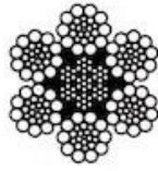
6 x 26 WARRINGTON SEALE WITH IWRC
