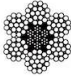
6 x 25 FILLER WIRE WITH IWRC
