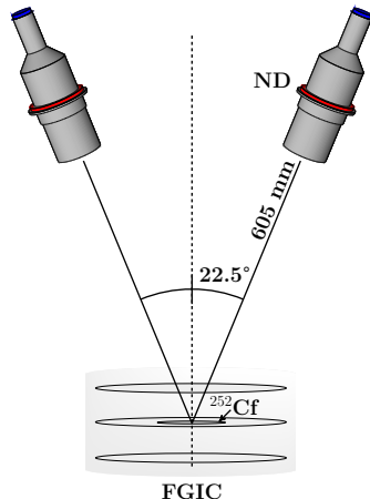
Figure: Illustration of the experimental setup. On the left-hand side, a photo taken from behind the neutron detector arrays is shown. The right-hand side shows a cross-section through the setup, where relevant dimensions are given.
