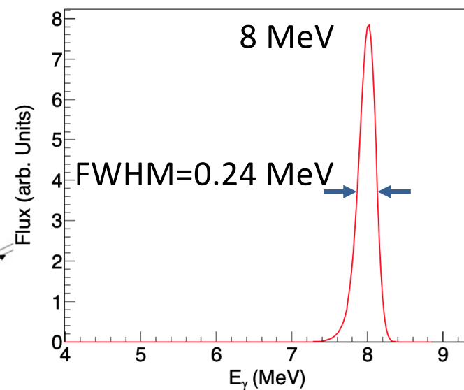
Example \gamma -ray Beam Spectrum
