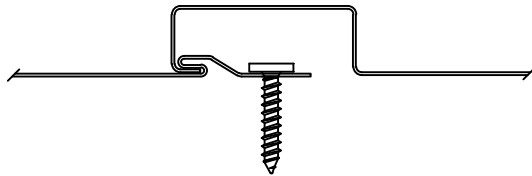
PF BOARD and BATTEN SEAM
