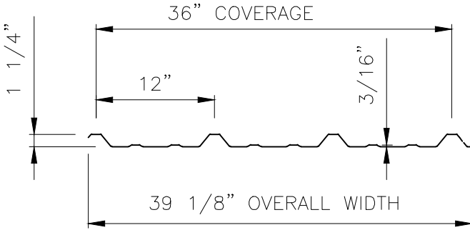
PF-12-36 PROFILE - ROOFS (Purlin Bearing Leg)
