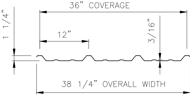
PF-12-36 PROFILE - WALLS (Non-Purlin Bearing Leg)
