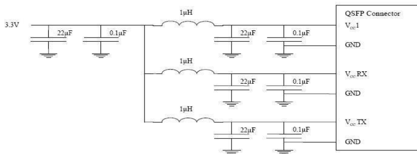
Figure 4. Host Board Power Supply Filtering
