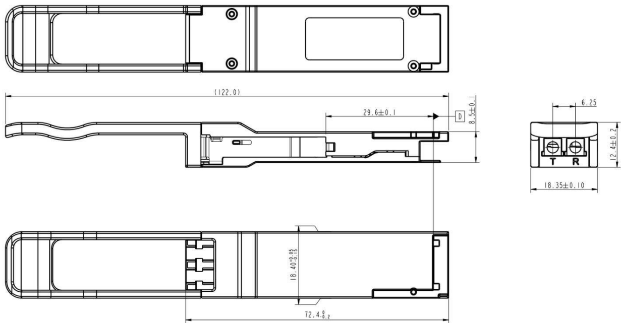
Figure 9 . Mechanical Specifications
