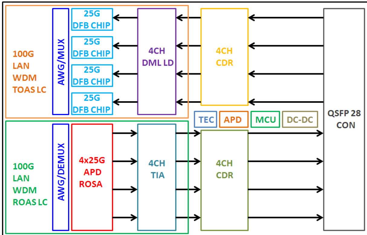
Figure1.Module Block Diagram
