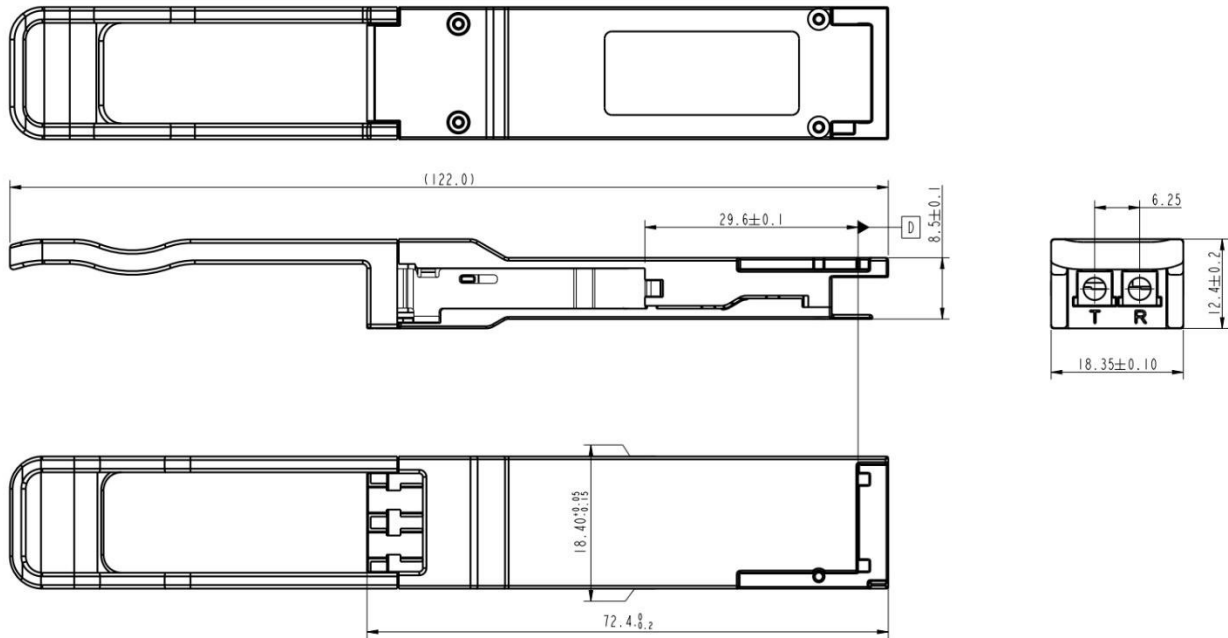
Figure 3. Mechanical Dimensions
