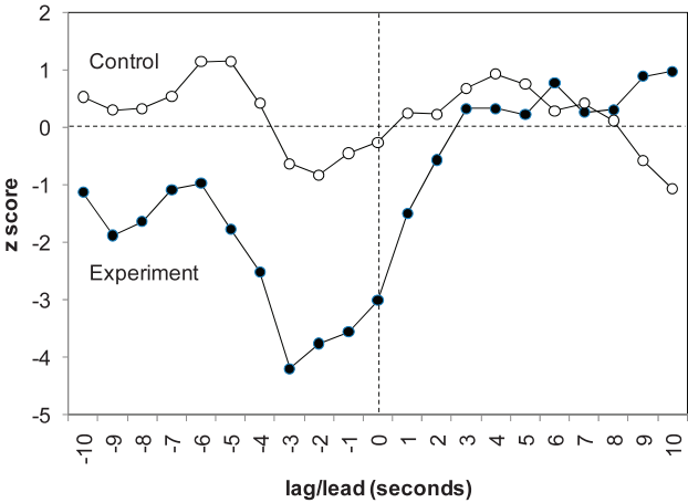
FIG. 7. (Color online) Lag/lead analysis for residuals.
