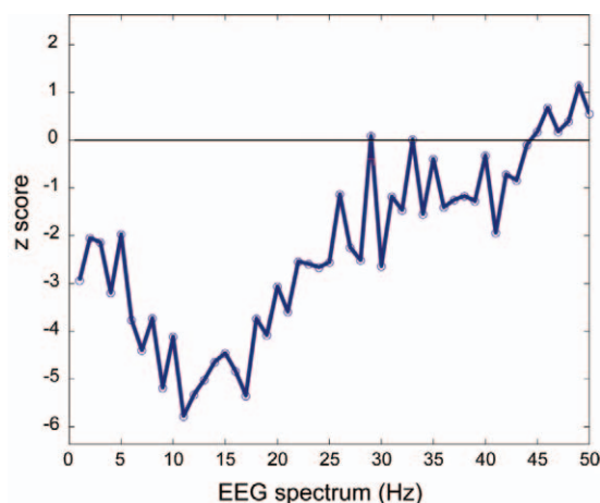
FIG. 13. (Color online) Drop in EEG spectral power when comparing attention-toward versus attention-away conditions across all sessions, in terms of standard normal deviates. Notice the particularly strong drop around the \alpha band (8–12 Hz).
