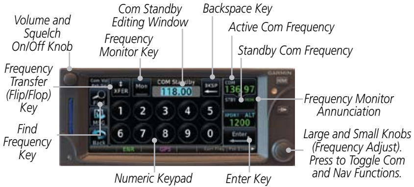
Figure 3-1 Nav/Com Controls
